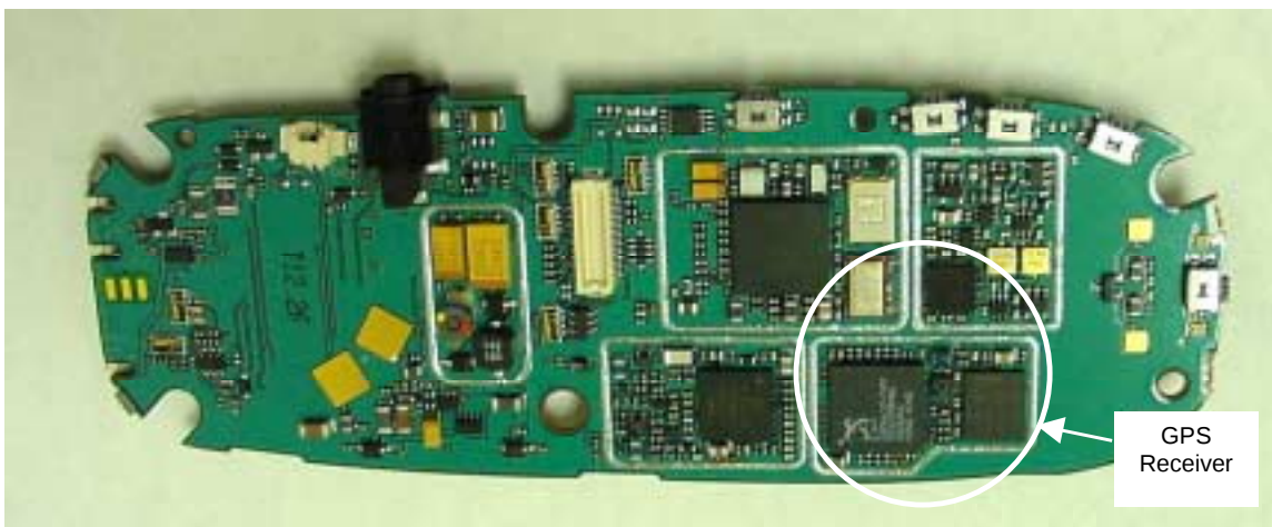
Figure 9-1-1. Photograph of frontside of printed wiring assembly.
