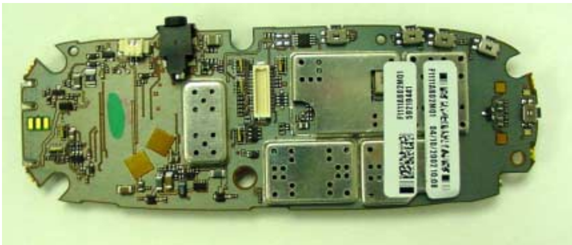
Figure 9-1-1. Photograph of frontside of printed wiring assembly.
