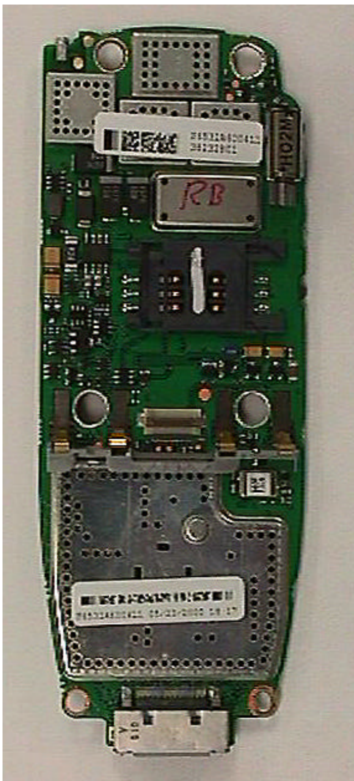
Photograph 9-2: Back side of the radio main board.
