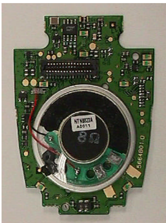
Photograph 9-4: Front side of keypad board, showing attached speaker.
