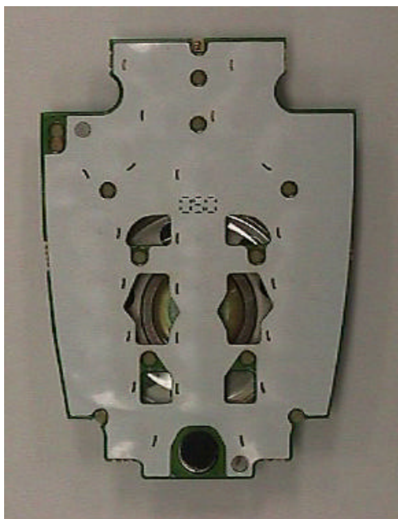
Photograph 9-3: Front side of keypad board.
