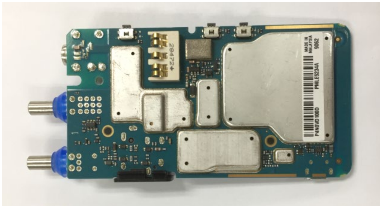
RF board with Shields (Top)
