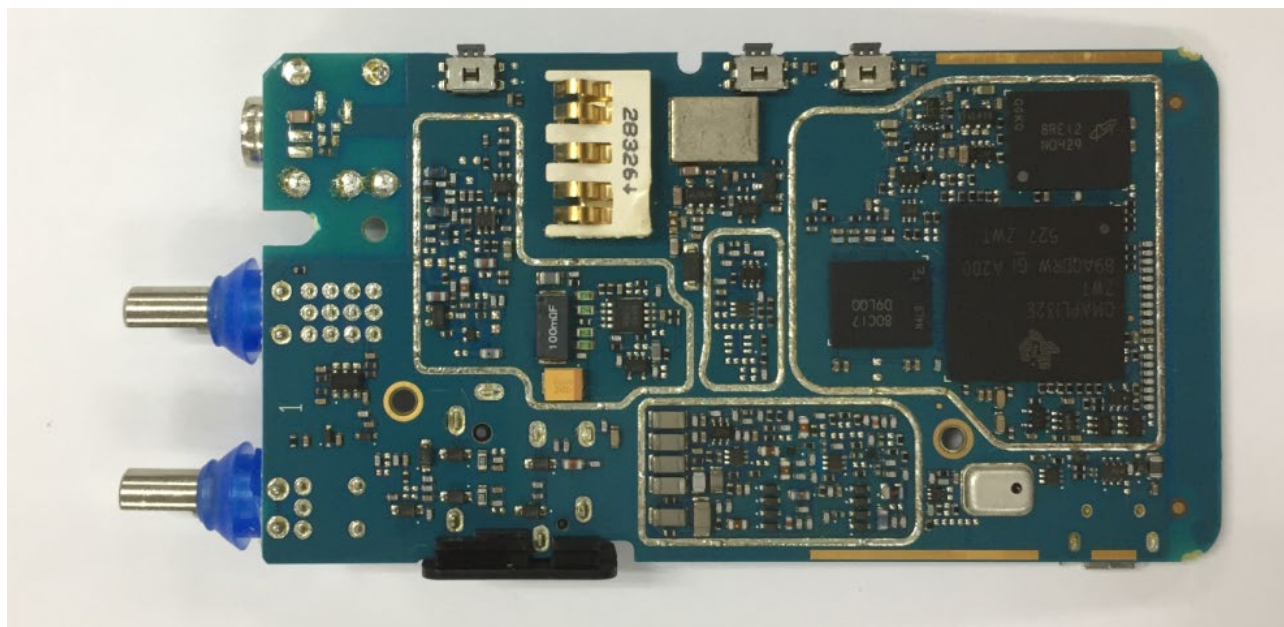
RF board without Shields (Top)
