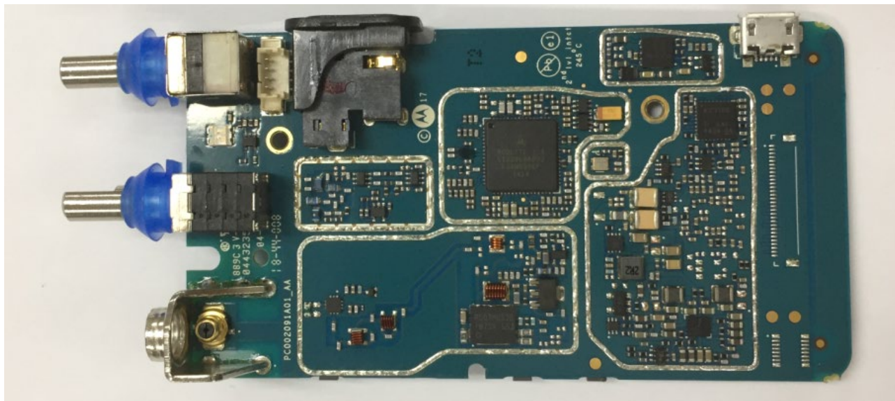
RF board without Shields (Bottom)
