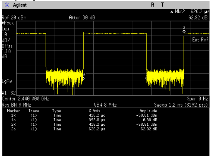
Duty Cycle
