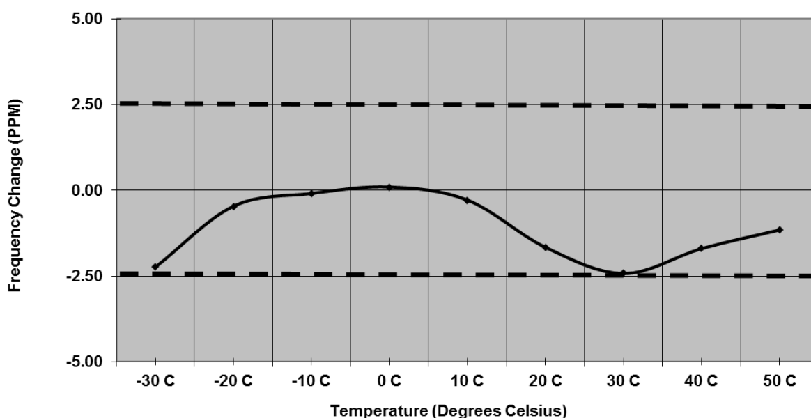
Figure 7.6.2-1: Frequency Stability – 462.6375 MHz
