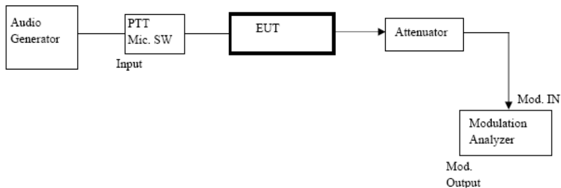
Figure 1. Modulation limiting setup
