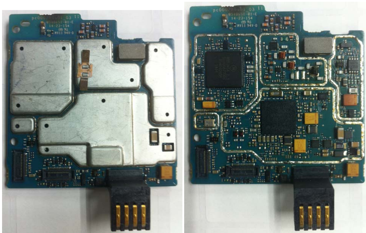
RF board with and without Shields (Top)
