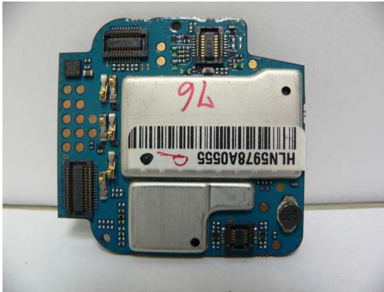
11. Expander board with Shields (Bottom).
