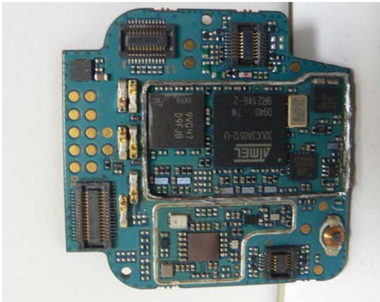
12. Expander board without Shields (Bottom).
