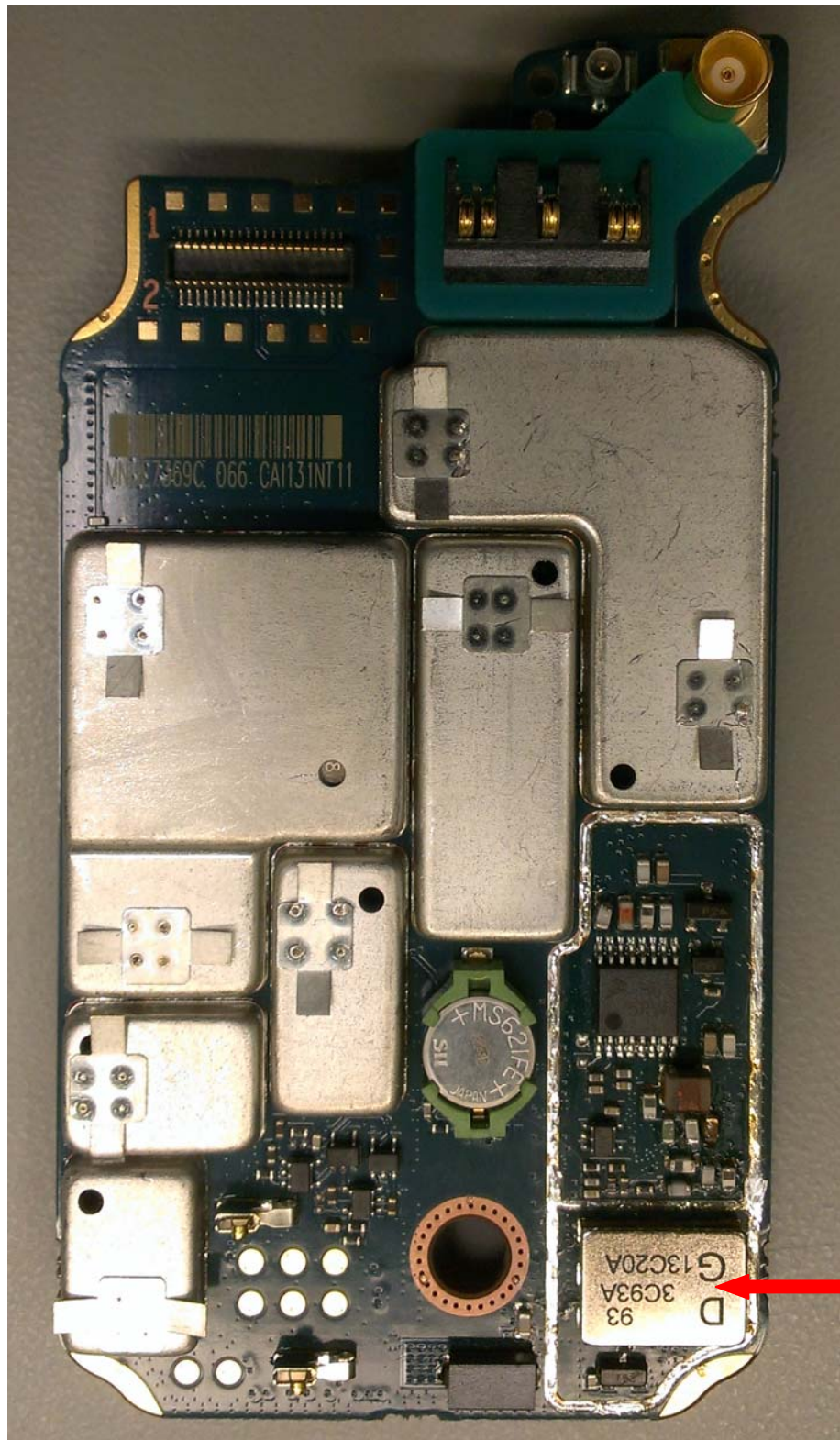
RF board without shields (Top)
