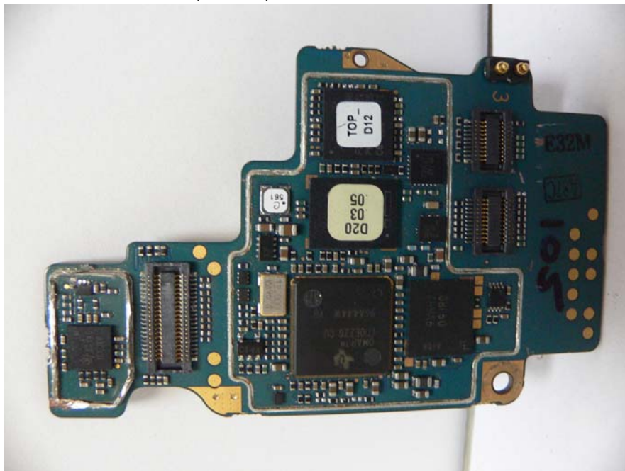
8. Vocon board without Shields (Bottom).
