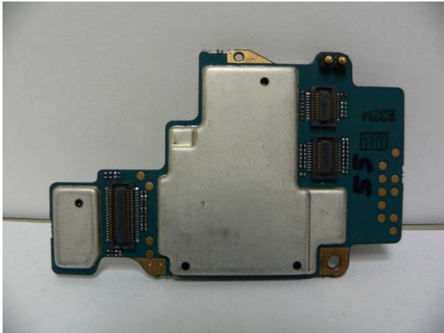
7. Vocon board with Shields (Bottom).
