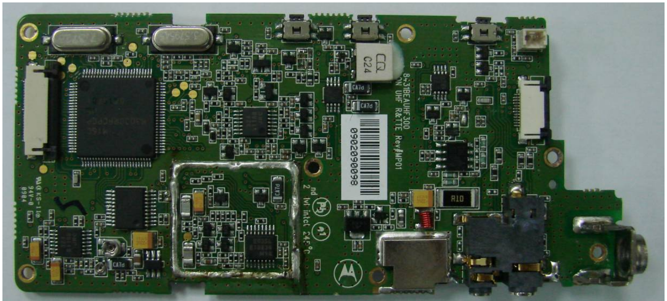
Figure 9-2: Top Side of PCB (without shield)
