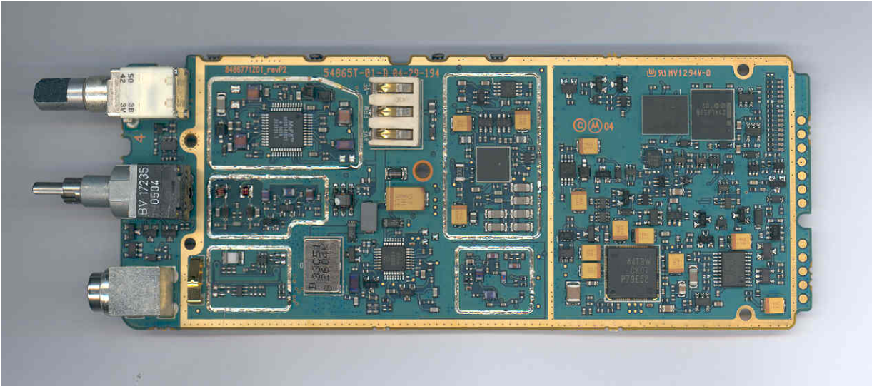
Figure 9-4: Bottom Side of PCB (without shields)
