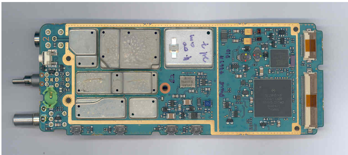
Figure 9-1: Top Side of PCB (with shields)
