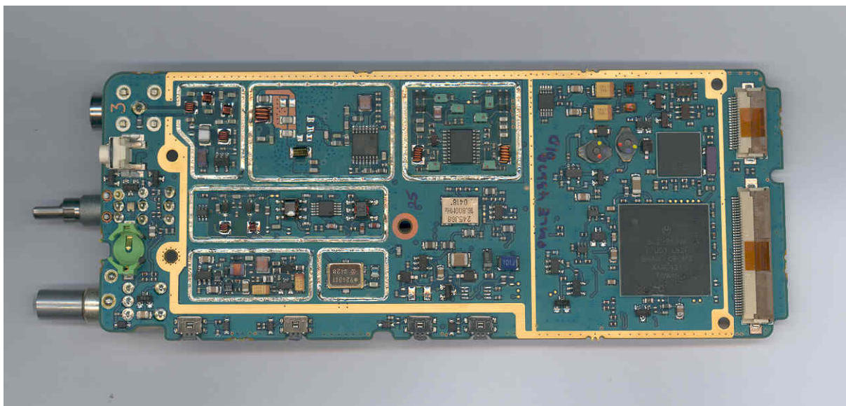
Figure 9-2: Top Side of PCB (without shields)
