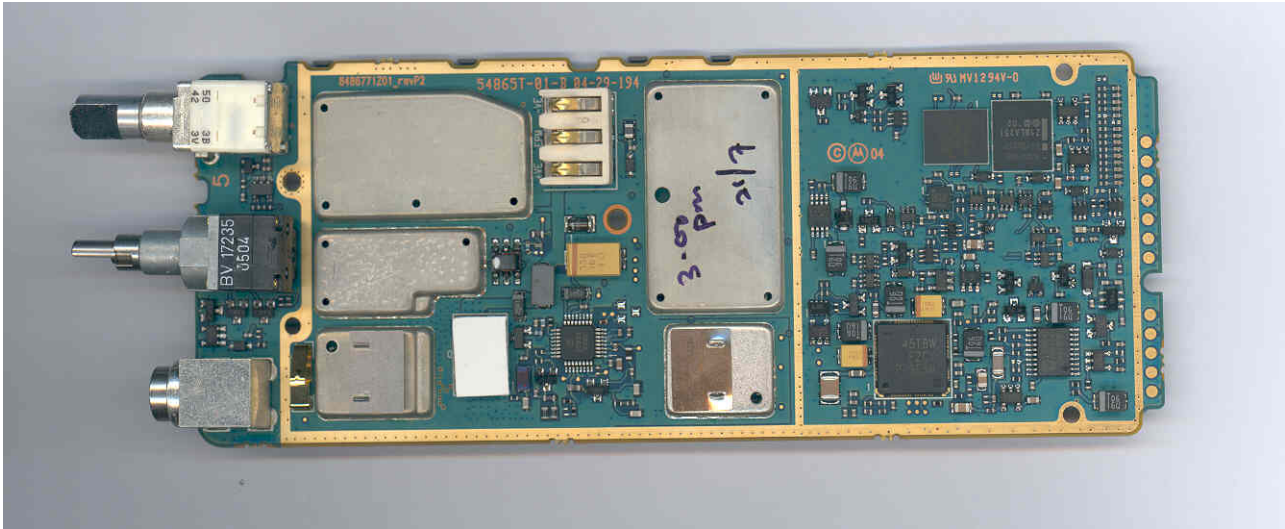
Figure 9-3: Bottom Side of PCB (with shields)
