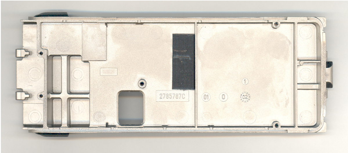
Figure 9-6: Bottom View of chassis.
