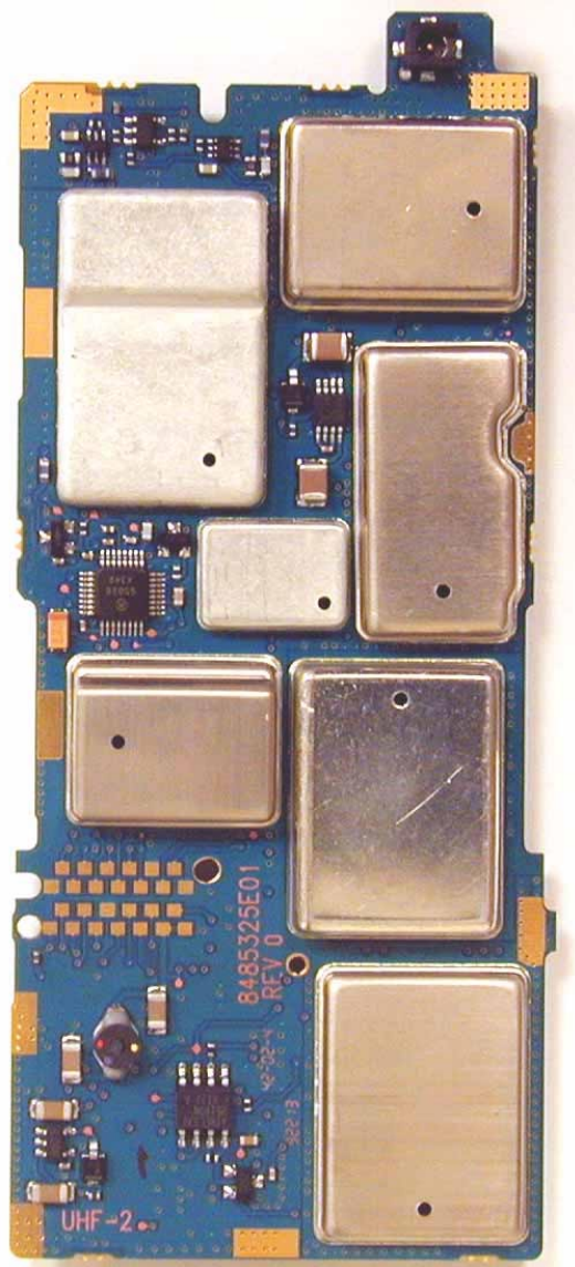
RF board with Shields (Top)
