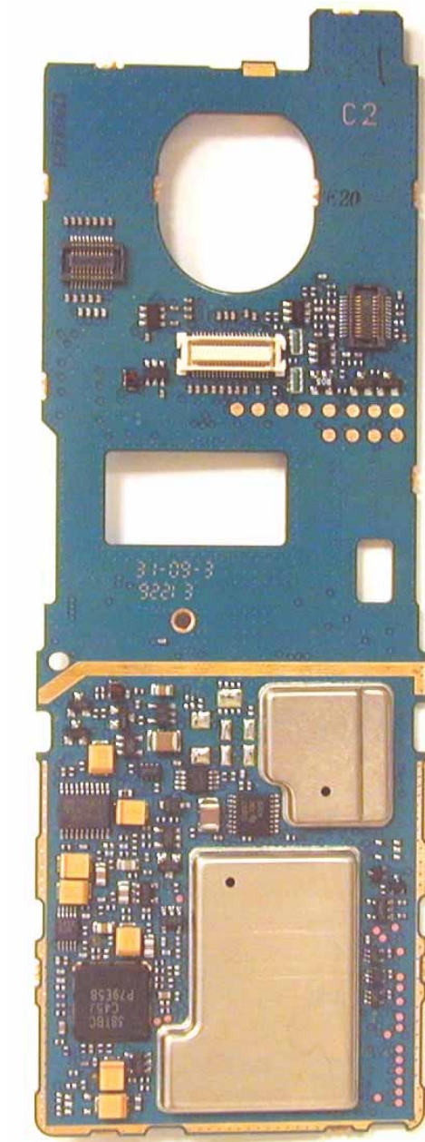
Vocon board with Shields (Top)
