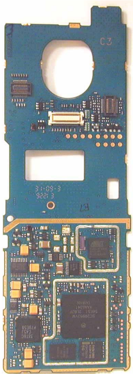
Vocon board without Shields (Top)
