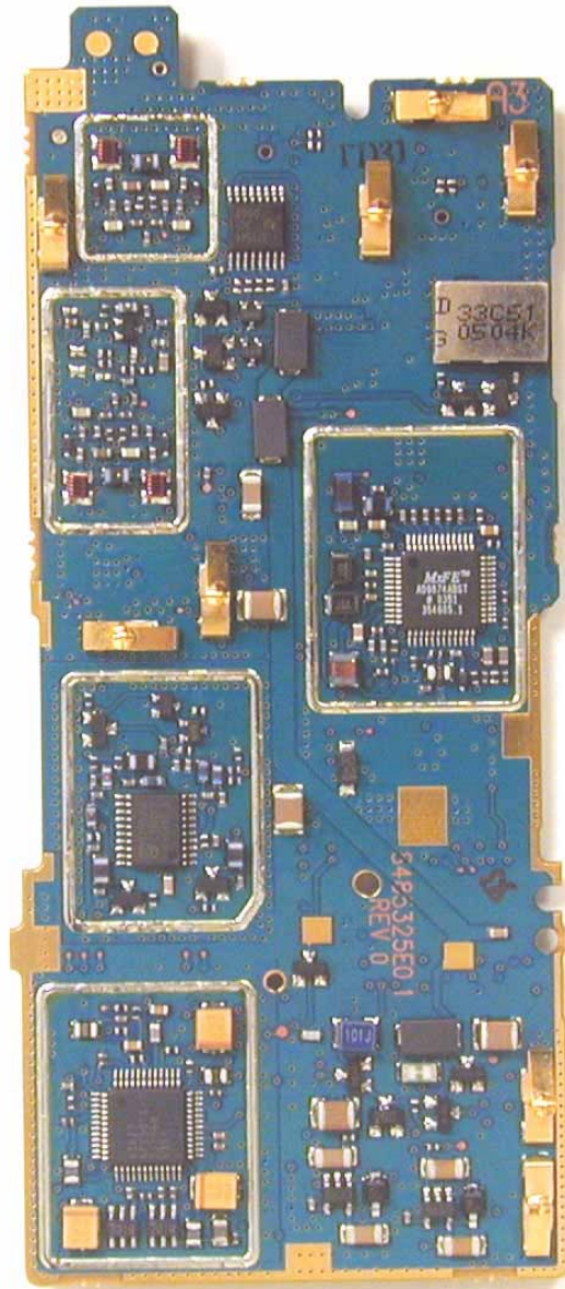
RF board without Shields (Bottom)
