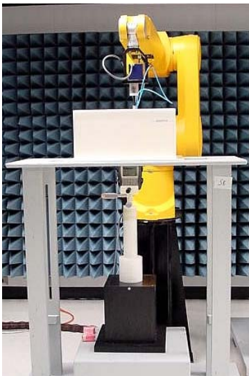
Figure 10: Robot Test Setup 2.4GHz band (Body)
