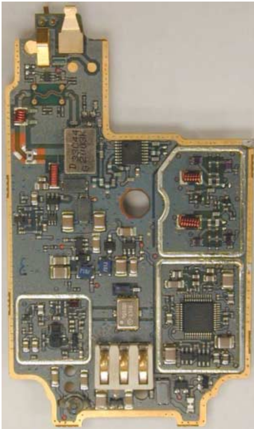
RF board without Shields (Bottom)
