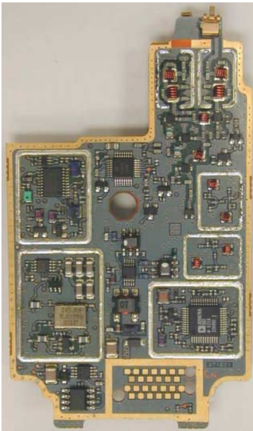
RF board without Shields (Top)
