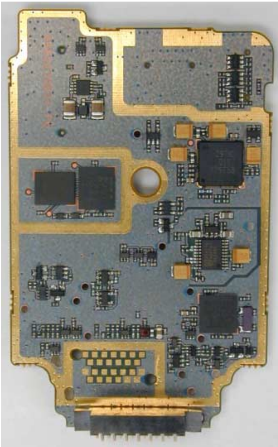
Vocon board (Bottom))
