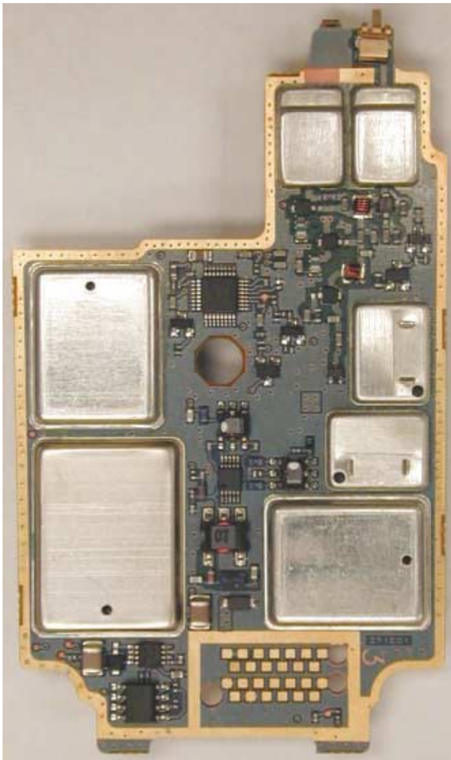
RF board with Shields (Top)
