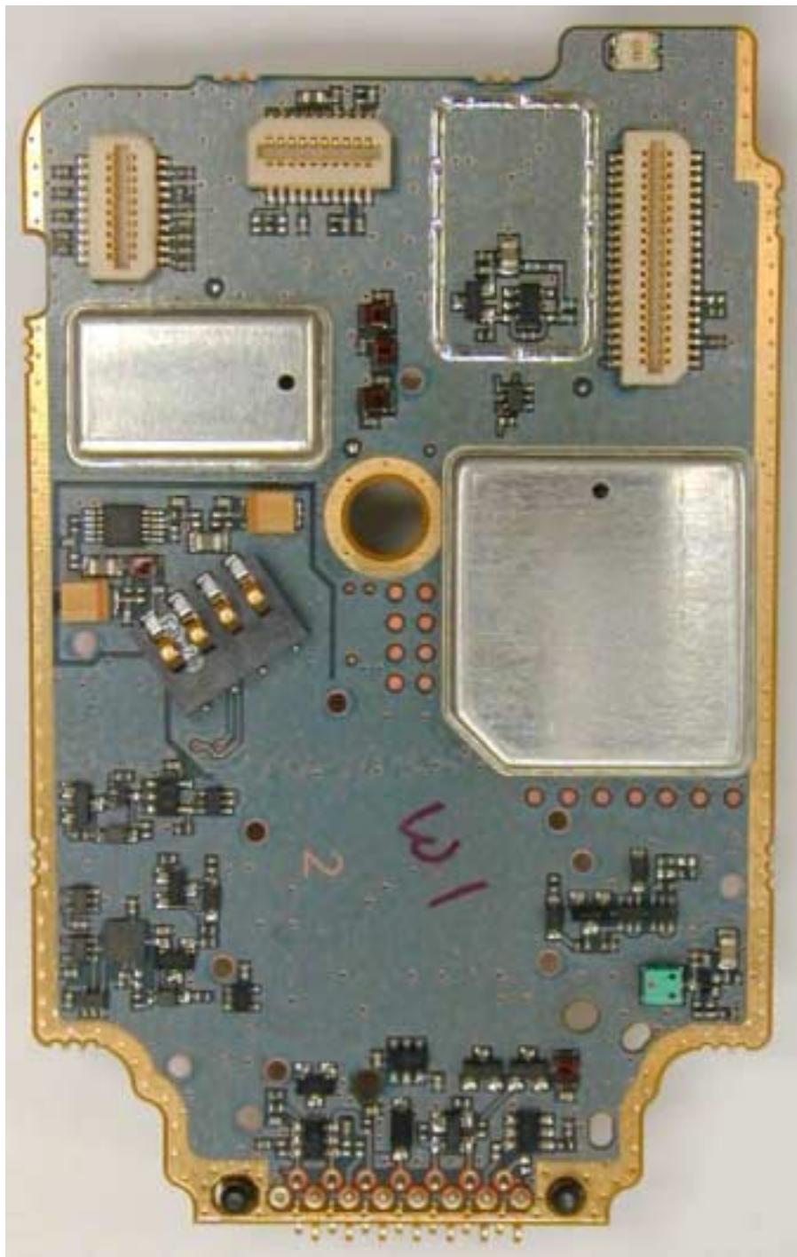
Vocon board with Shields (Top)
