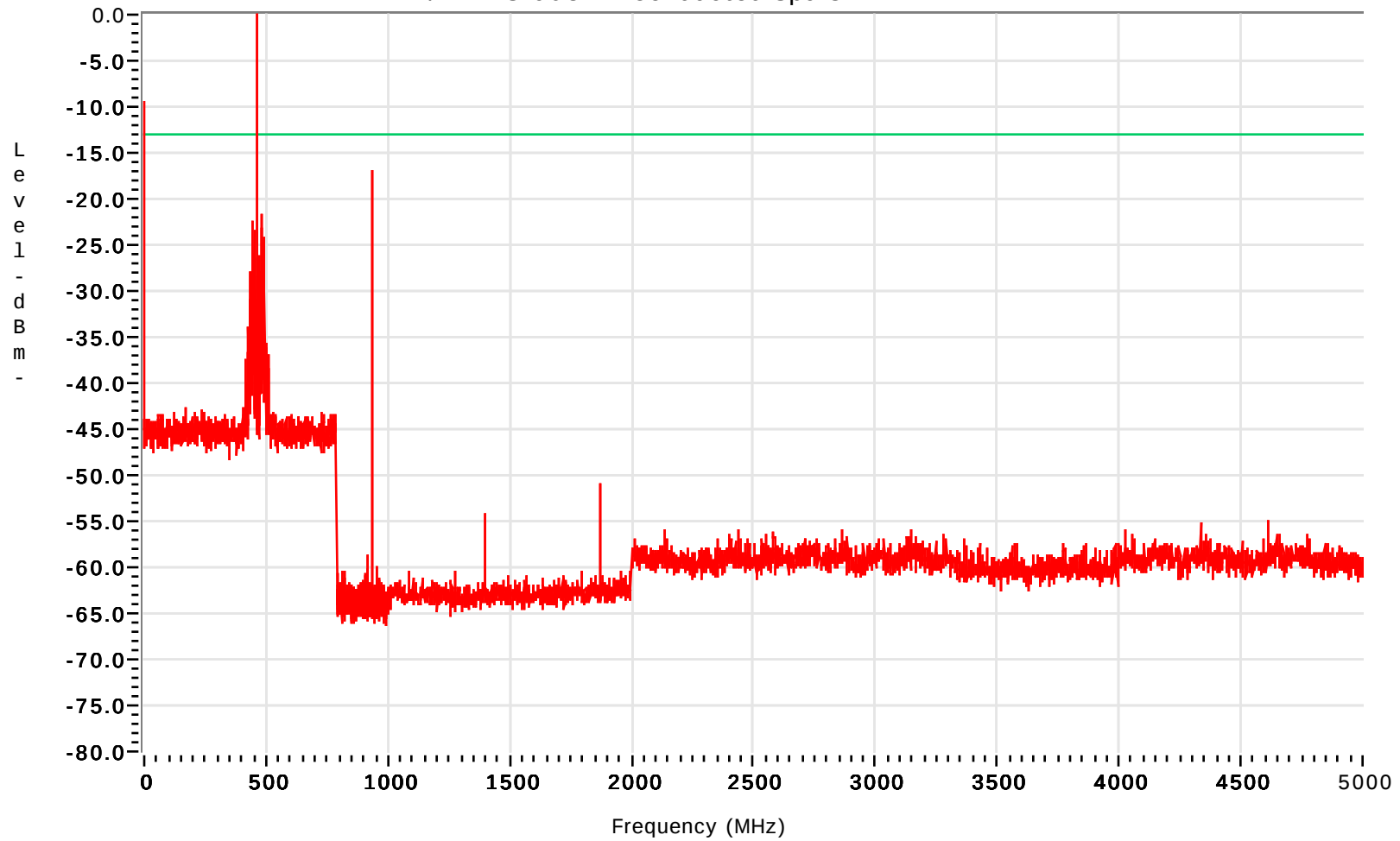
EIA/TIA RS-603 TX Conducted Spurs
