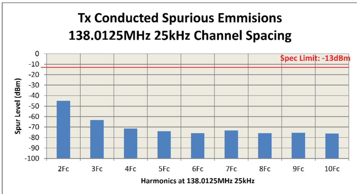
6G-2 – 138.0125MHz, 25kHz Channel Spacing, 3.3W (Not for FCC review)
