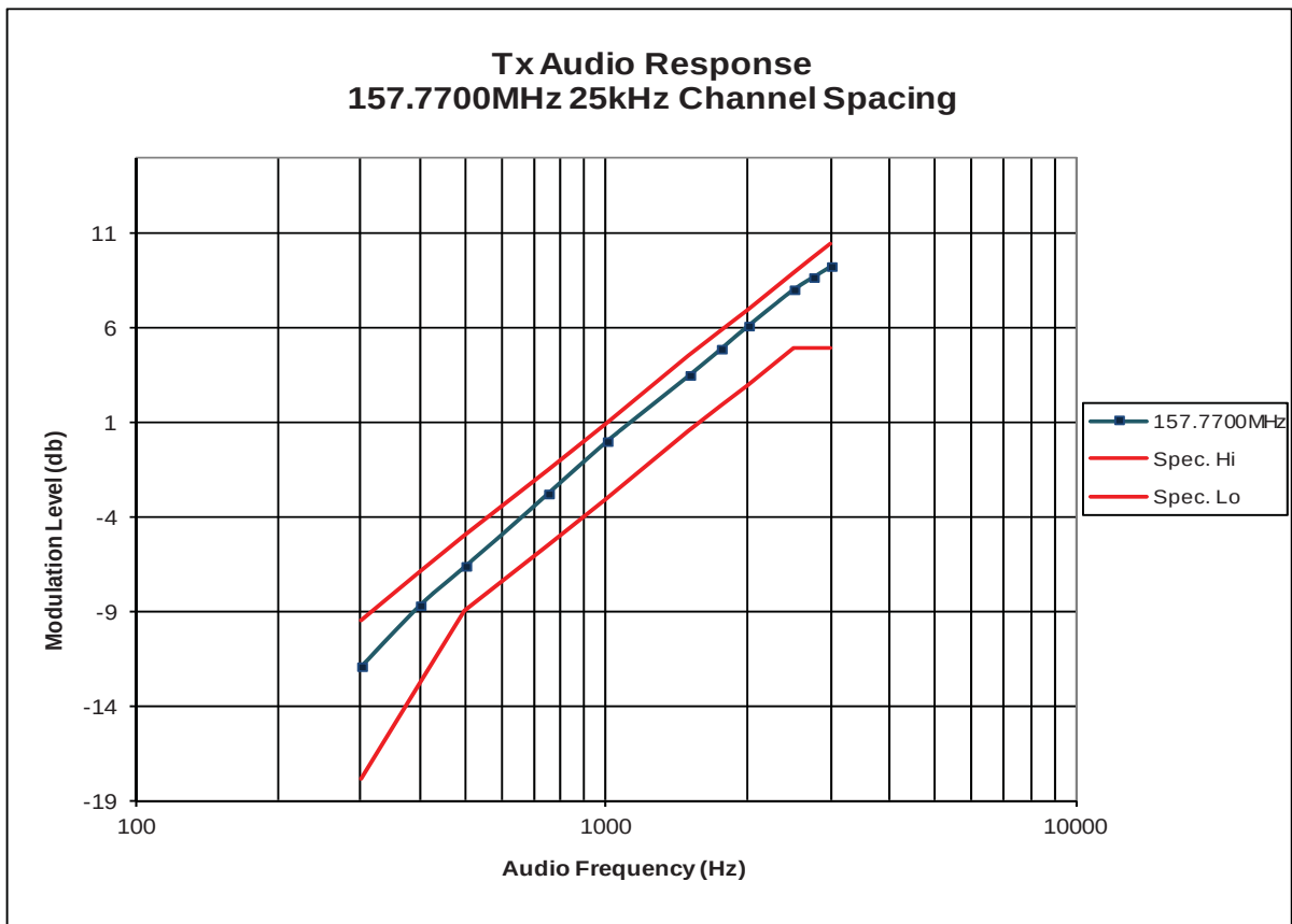
6B-3 –157.7700MHz, 25kHz Channel Spacing (Part22)
