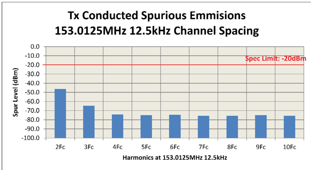
6G-3 – 153.0125MHz, 12.5kHz Channel Spacing, 3.3W
