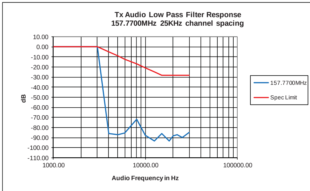
6C-3 –157.7700MHz, 25kHz Channel Spacing (Part22)
