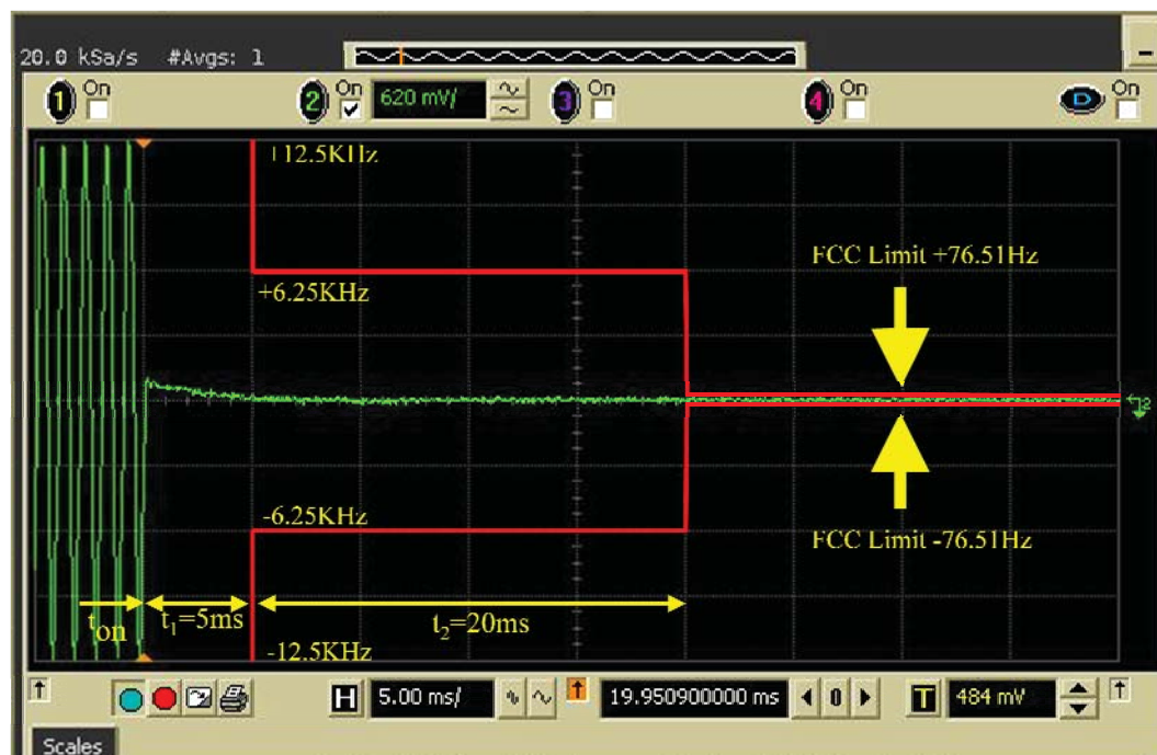
6I-1 – 153.0125MHz, 12.5kHz Channel Spacing – Transmitter On
