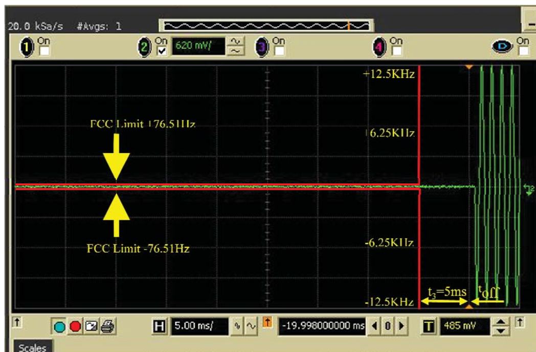
6I-2 – 153.0125MHz, 12.5kHz Channel Spacing – Transmitter Off
