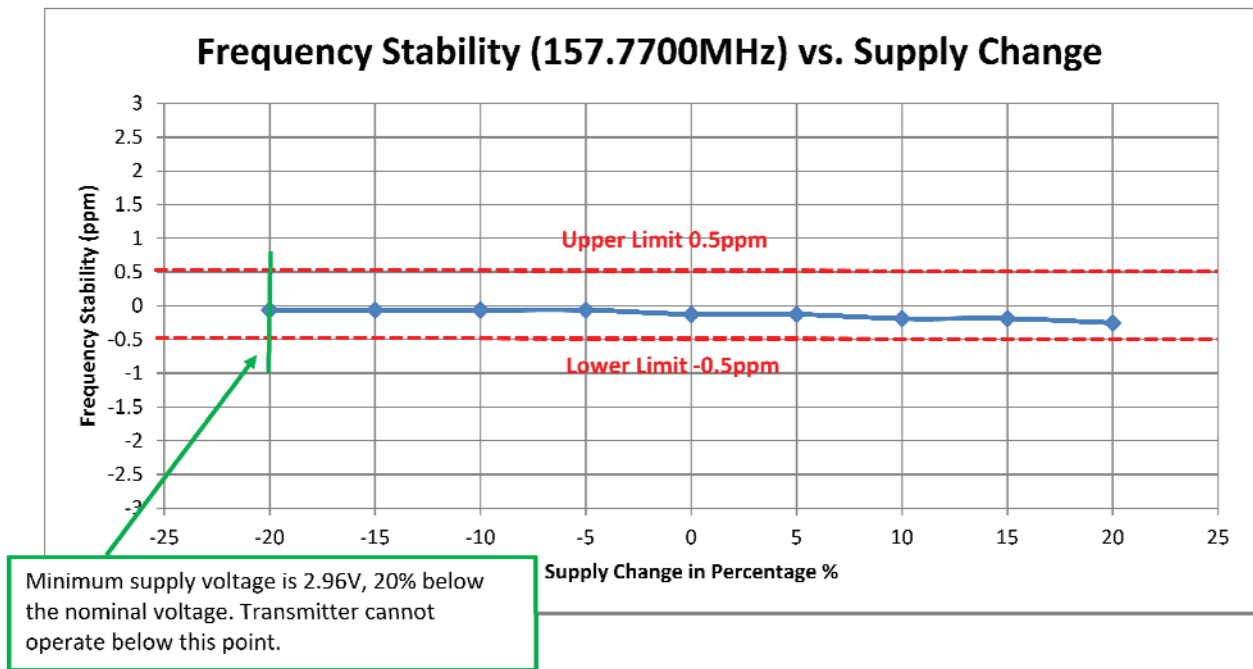
6H-4 – 157.77 MHz, Frequency Stability vs. Supply Voltage (Part 22)
