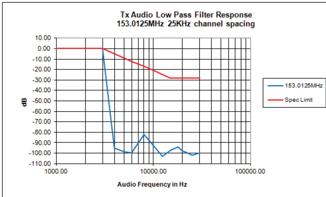
6C-2 –153.0125MHz, 25kHz Channel Spacing (Not for FCC review)
