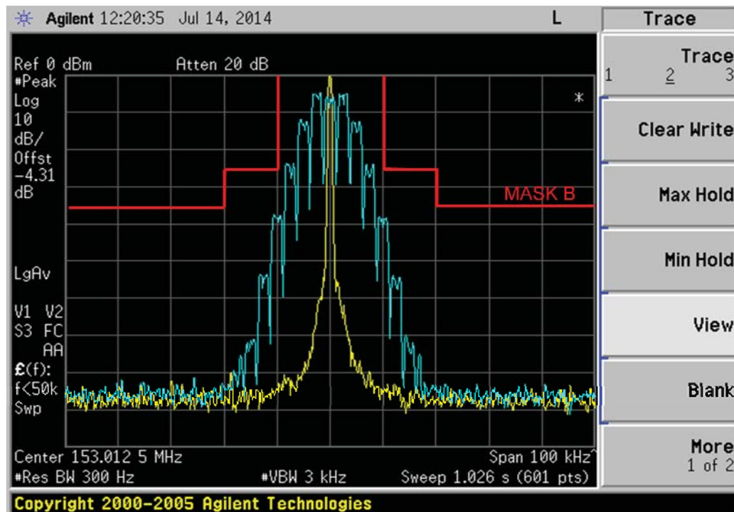
6E-6: 153.0125MHz, 25kHz, 2500Hz Audio and DPL Tone Modulation, 16K0F3E Mask B (Not for FCC review)
