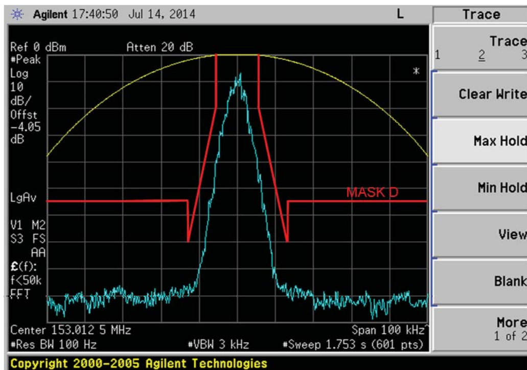
6E-8: 153.0125MHz, O.153 Test Pattern 4FSK Voice (F2 Silent) Modulation, 7K60FXE Mask D
