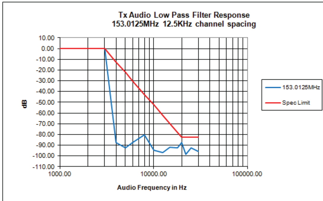
6C-1 –153.0125MHz, 12.5kHz Channel Spacing
