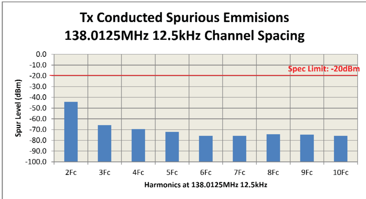
6G-1 – 138.0125MHz, 12.5kHz Channel Spacing, 3.3W (Not for FCC review)
