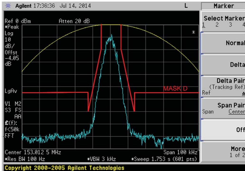
6E-7: 153.0125MHz, O.153 Test Pattern 4FSK Data (F2 BER) Modulation, 7K60FXD Mask D
