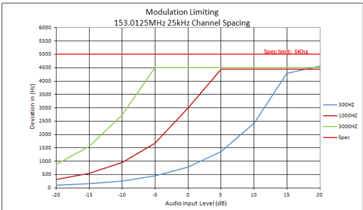
6D-2 –153.0125MHz, 25kHz Channel Spacing (Not for FCC review)
