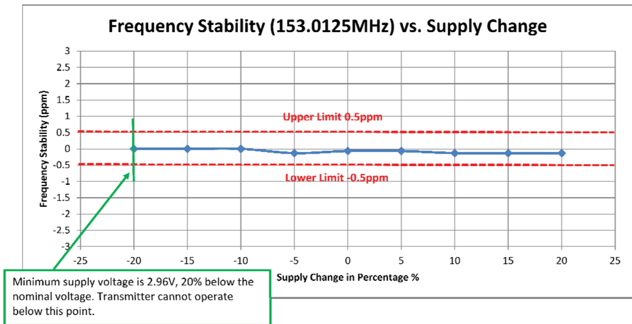
6H-2 – 153.0125MHz, Frequency Stability vs. Supply Voltage
