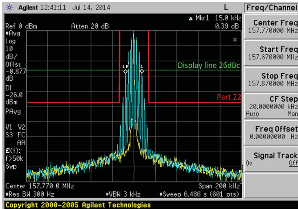
6E-10: 157.770MHz, 25kHz, 2500Hz Audio Modulation Only, 16K0F3E (Part 22)
