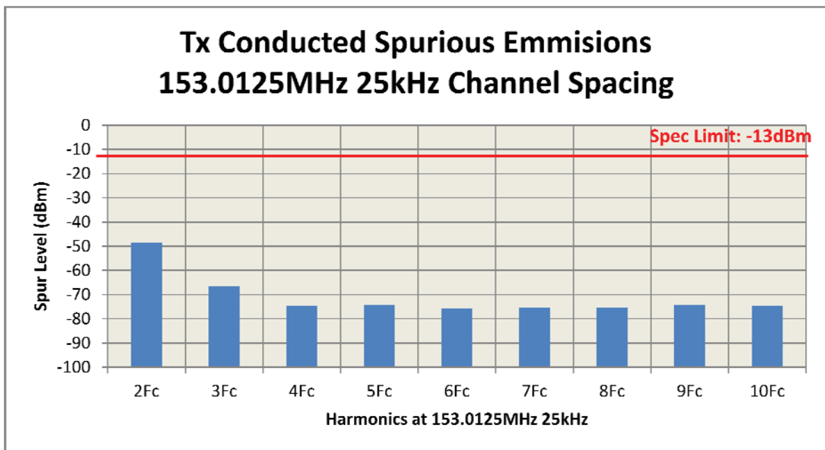
6G-4 – 153.0125MHz, 25kHz Channel Spacing, 3.3W (Not for FCC review)
