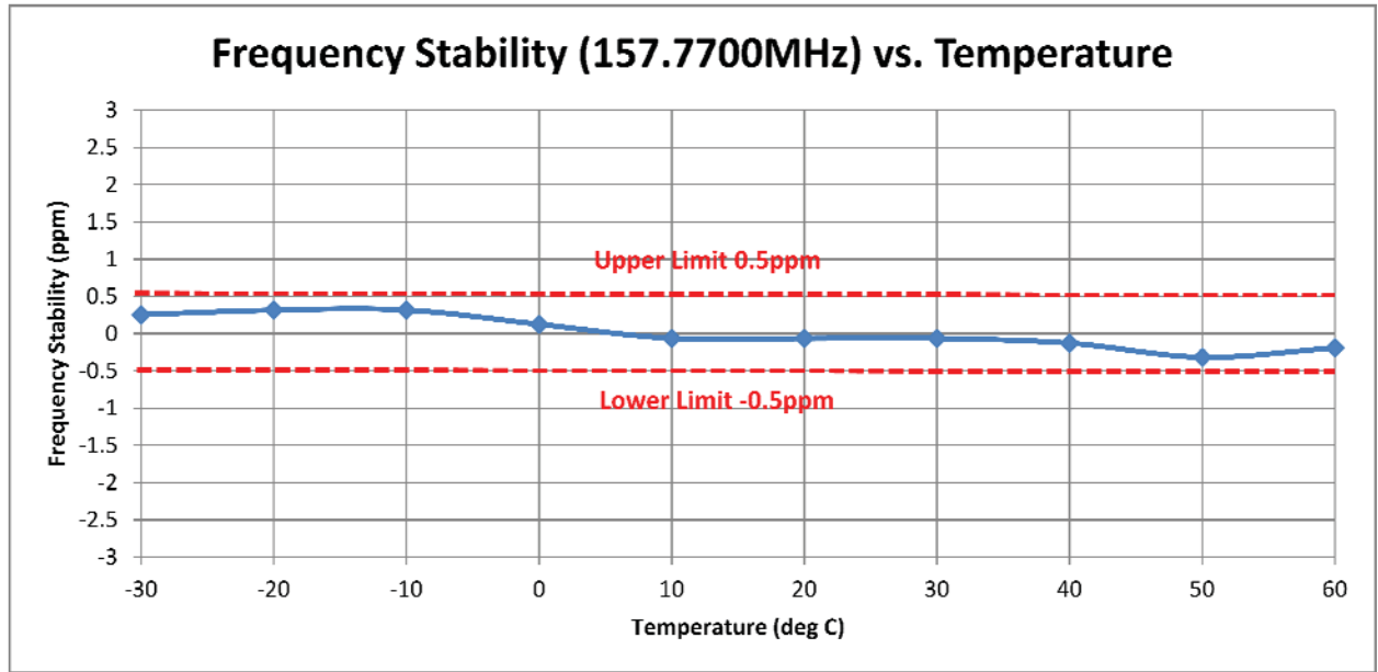
6H-3 – 157.77 MHz, Frequency Stability vs. Temperature (Part 22)
