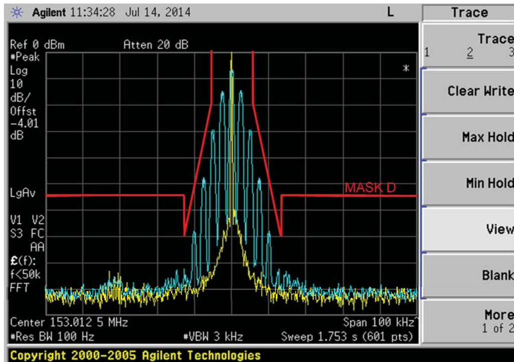
6E-3: 153.0125 MHz, 12.5kHz, 2500Hz Audio and PL Tone Modulation, 11K0F3E Mask D
