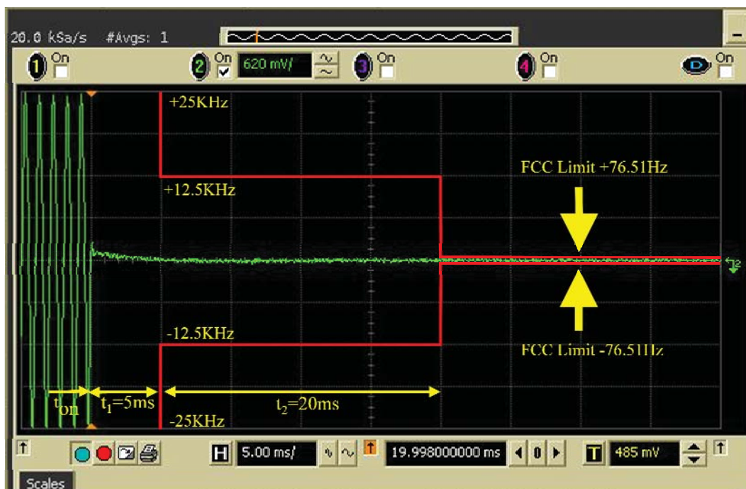
6I-3 – 153.0125MHz, 25kHz Channel Spacing – Transmitter On (Not for FCC review)
