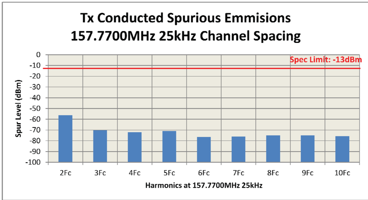
6G-5 – 157.7700MHz, 25kHz Channel Spacing, 3.3W (Part 22)
