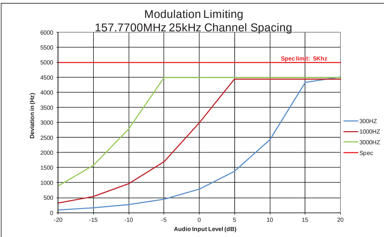
6D-3 –157.7700MHz, 25kHz Channel Spacing (Part22)
