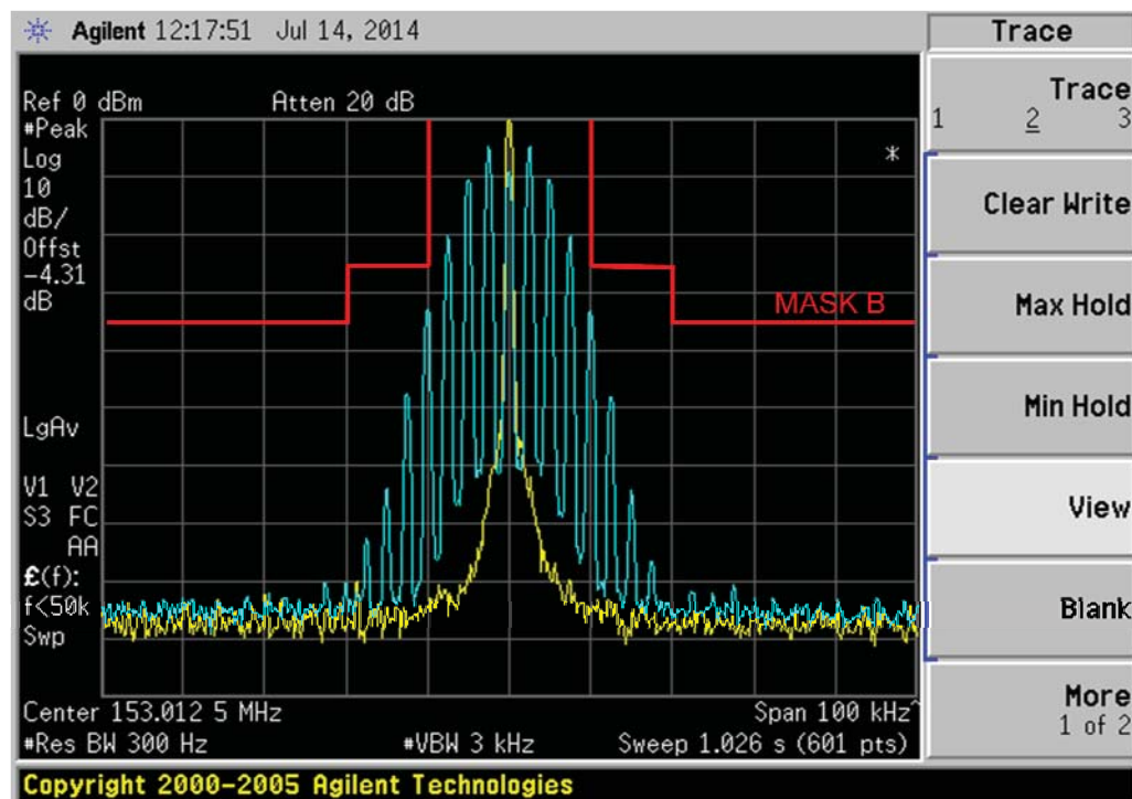
6E-2: 153.0125MHz, 25kHz, 2500Hz Audio Modulation Only, 16K0F3E Mask B (Not for FCC review)
