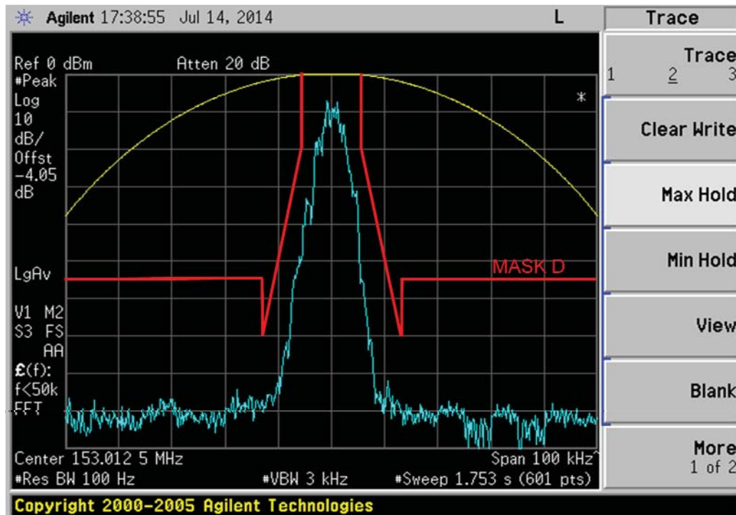
6E-9: 153.0125MHz, O.153 Test Pattern 4FSK Data (F2 BER) &amp; Voice (F2 Silent) Modulation, 7K60F1W Mask D
