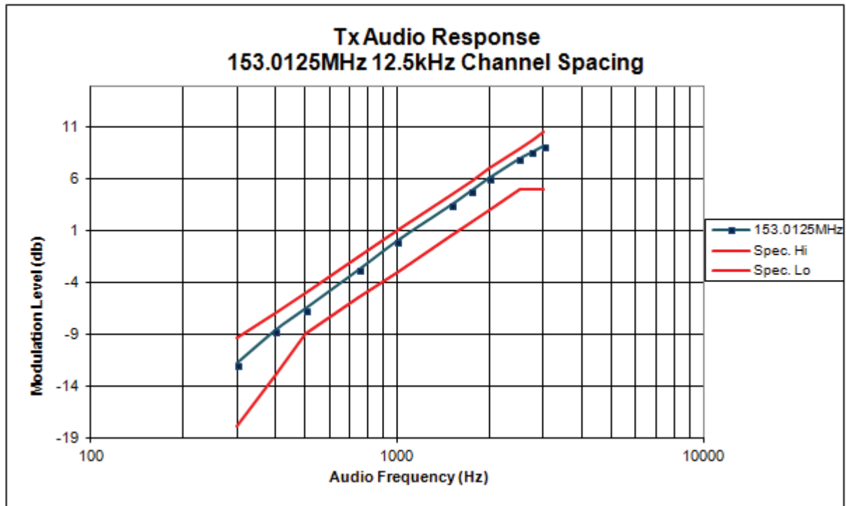
6B-1 –153.0125MHz, 12.5kHz Channel Spacing
