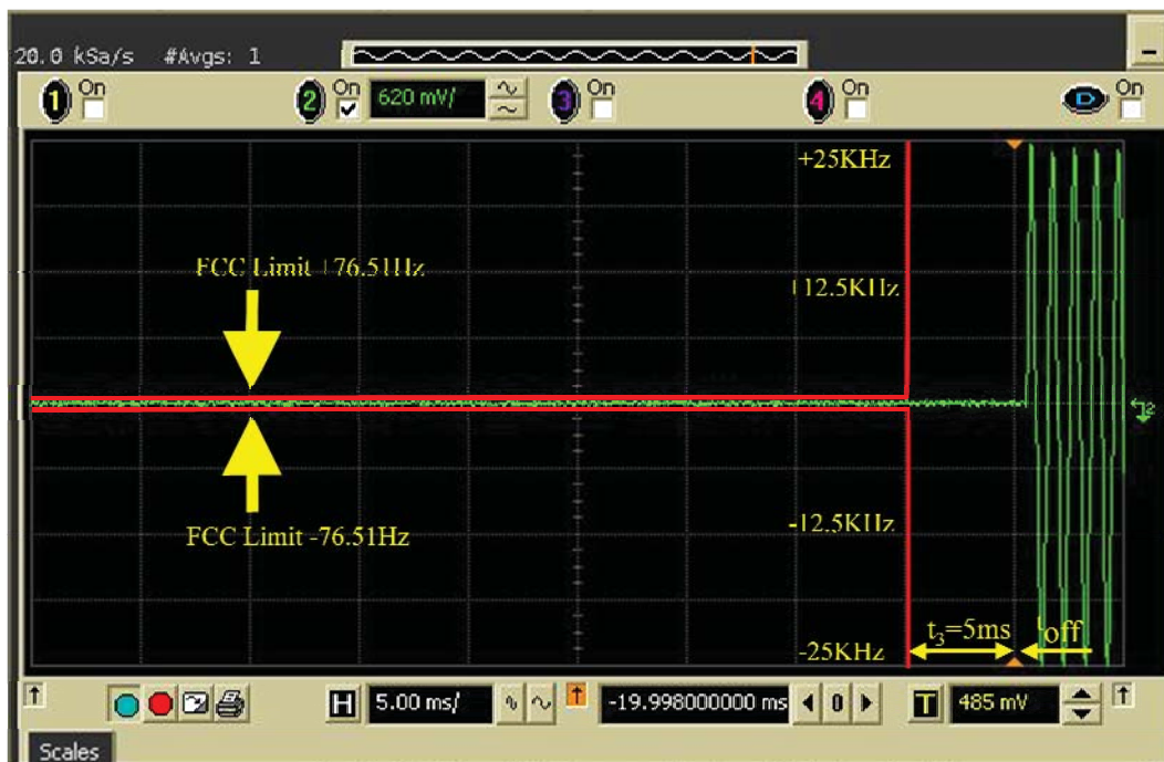
6I-4 – 153.0125MHz, 25kHz Channel Spacing – Transmitter Off (Not for FCC review)
