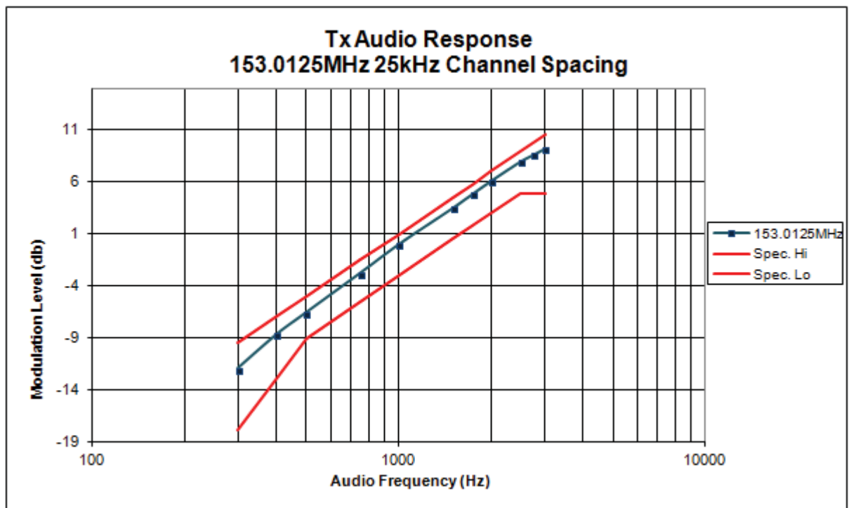
6B-2 –153.0125MHz, 25kHz Channel Spacing (Not for FCC review)
