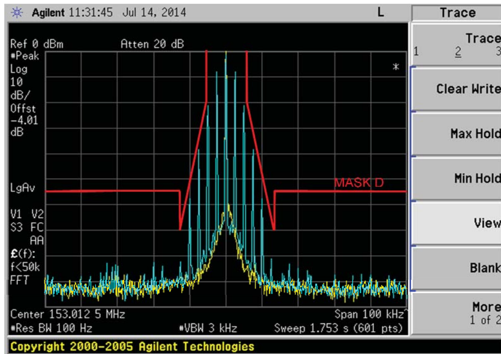
6E-1: 153.0125MHz, 12.5kHz, 2500Hz Audio Modulation Only, 11K0F3E Mask D
