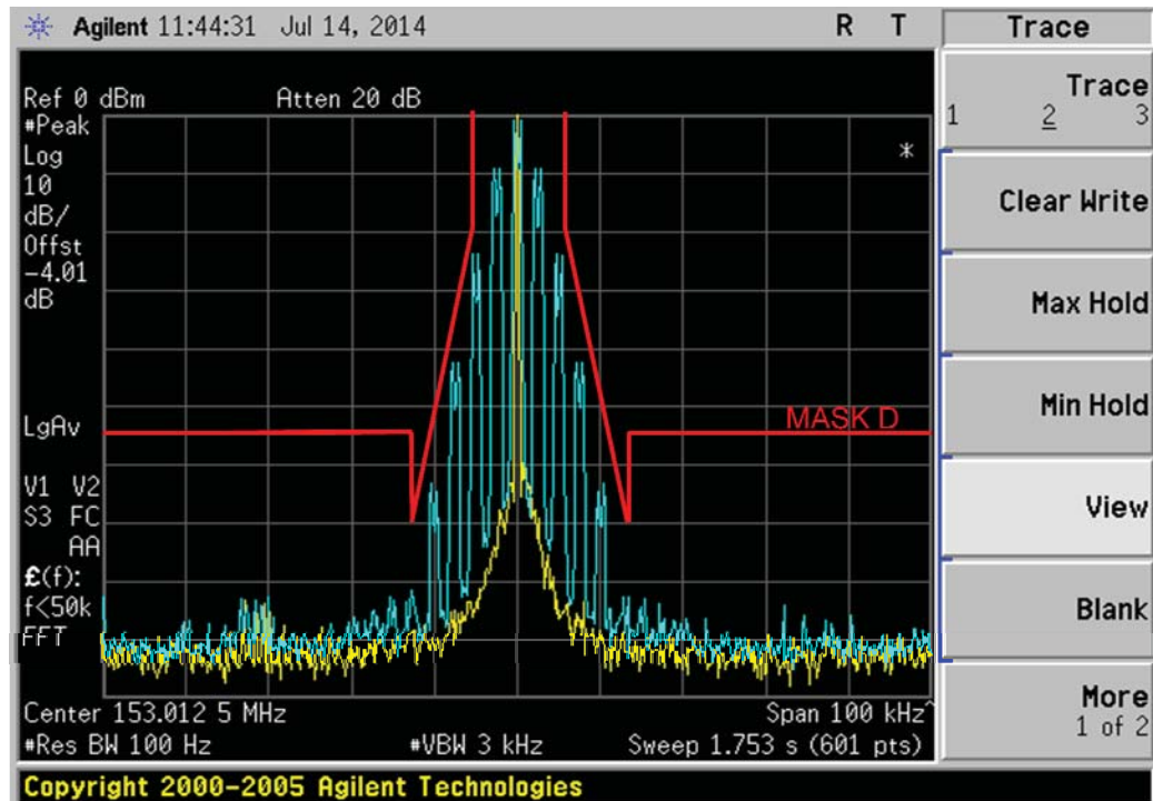
6E-4: 153.0125MHz, 12.5kHz, 2500Hz Audio and DPL Tone Modulation, 11K0F3E Mask D
