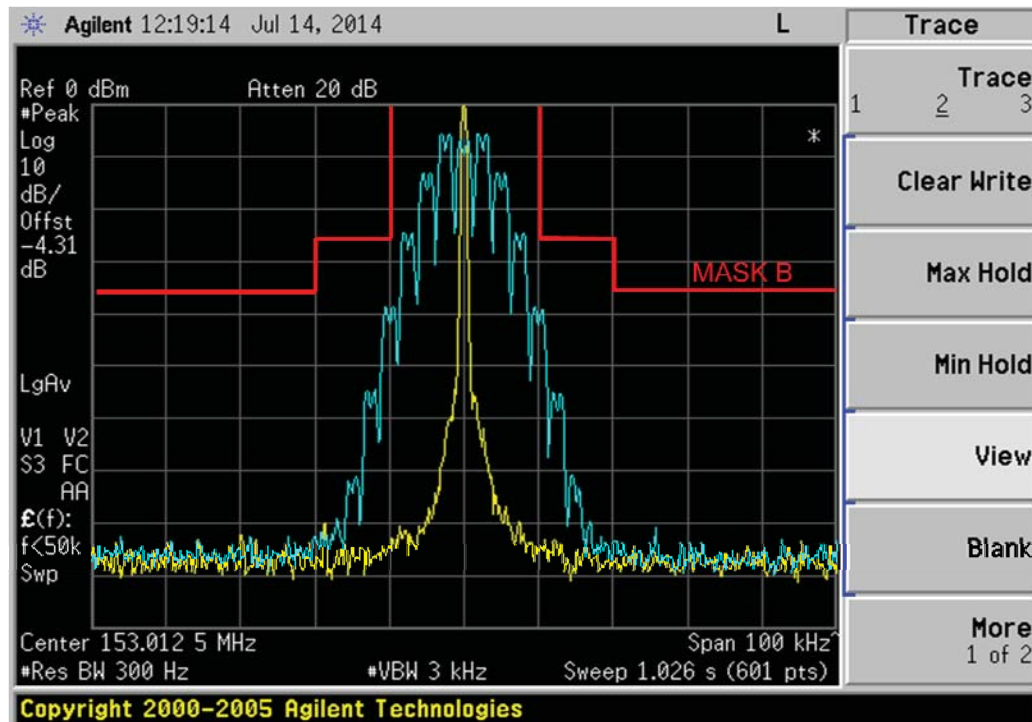
6E-5: 153.0125MHz, 25kHz, 2500Hz Audio and PL Tone Modulation, 16K0F3E Mask B (Not for FCC review)
