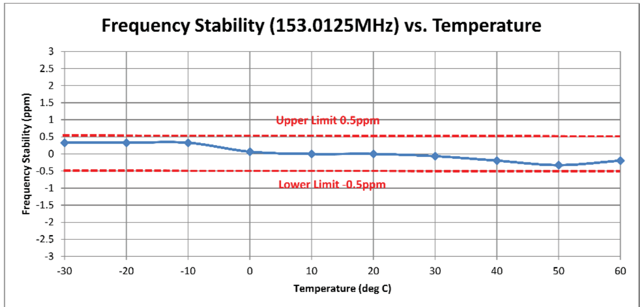
6H-1 – 153.0125MHz, Frequency Stability vs. Temperature
