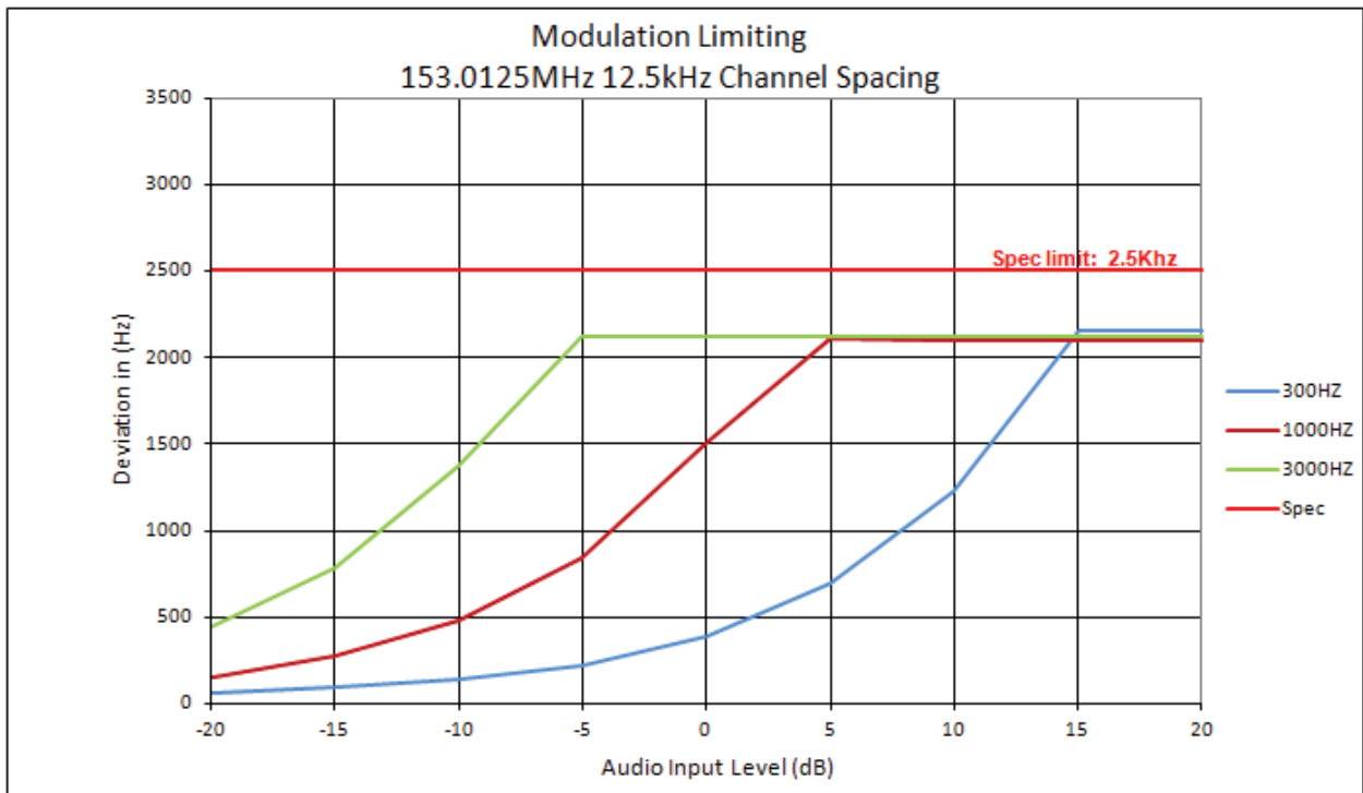
6D-1 –153.0125MHz, 12.5kHz Channel Spacing
