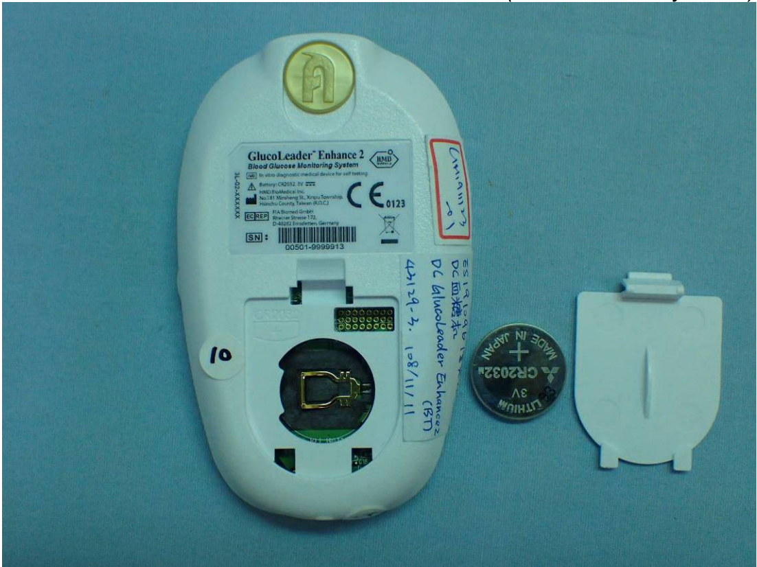
Figure 5 Internal View (Removed Battery Cover)
