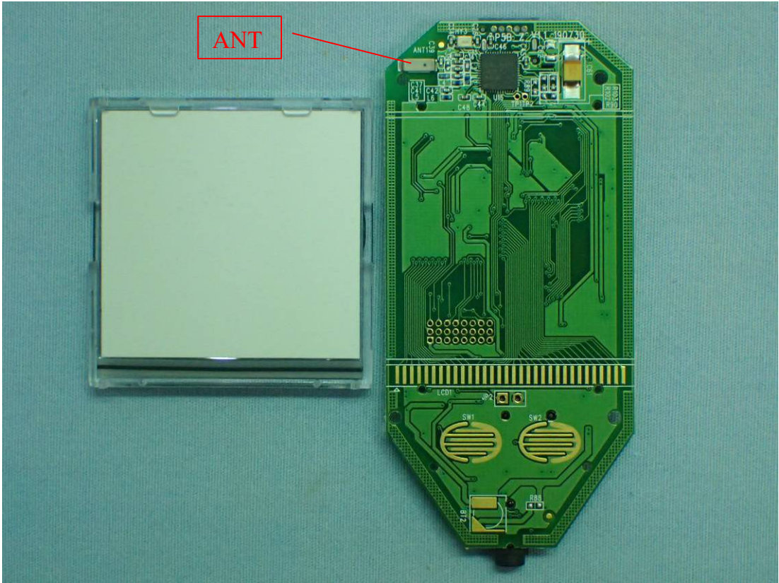
Figure 8 Internal View
