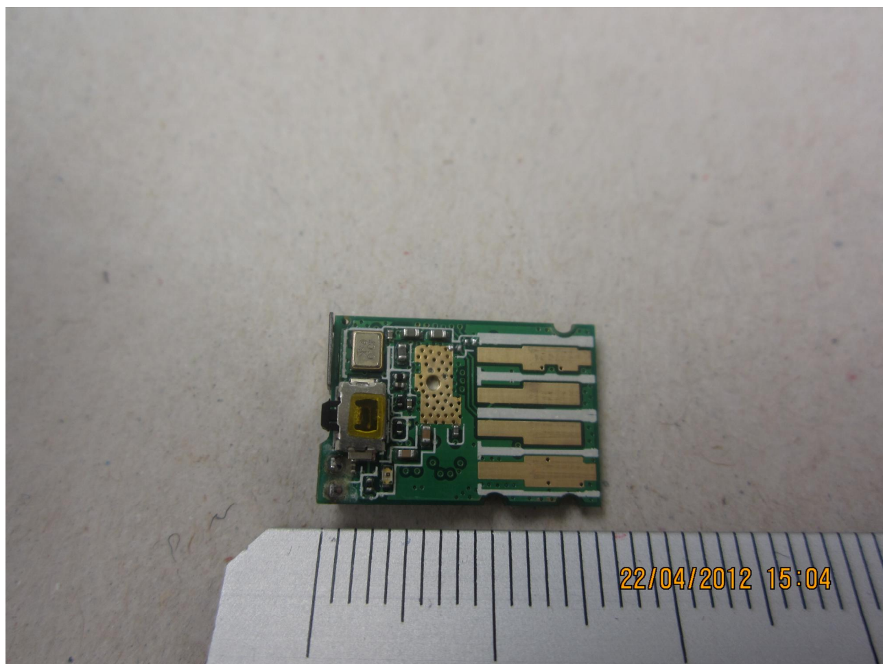
121150_28: USBN PCB bottom view
