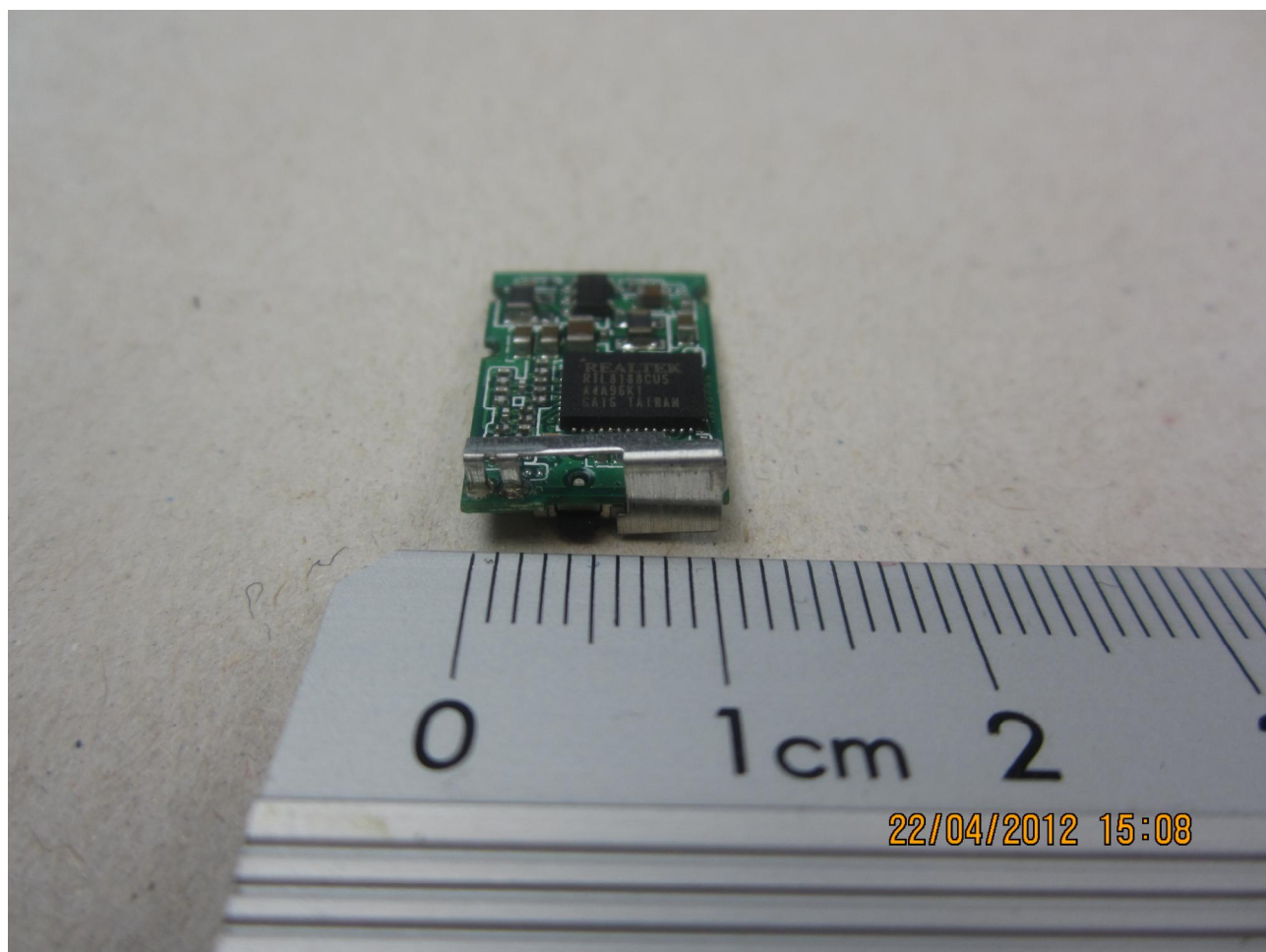
121150_30: USBN – internal antenna
