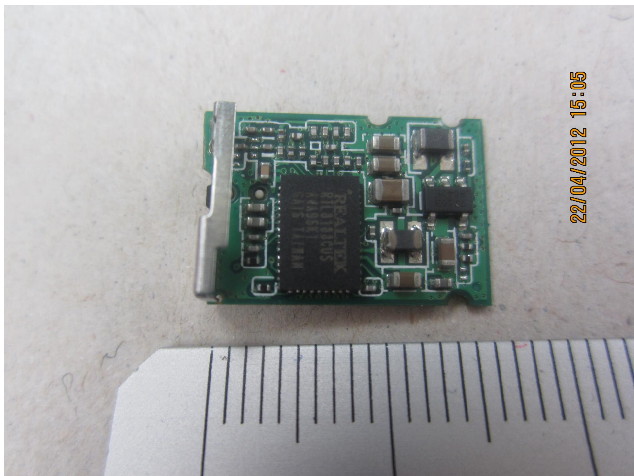
121150_29: USBN PCB top view
