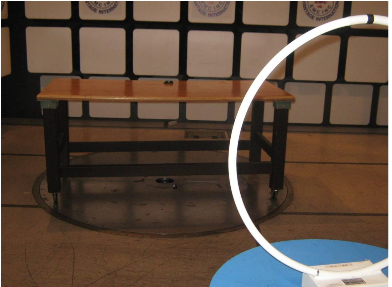
Radiated emissions testing (less than 30MHz)
