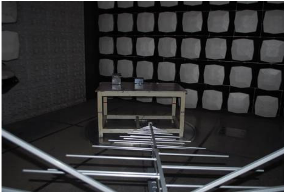
Radiated Emission
