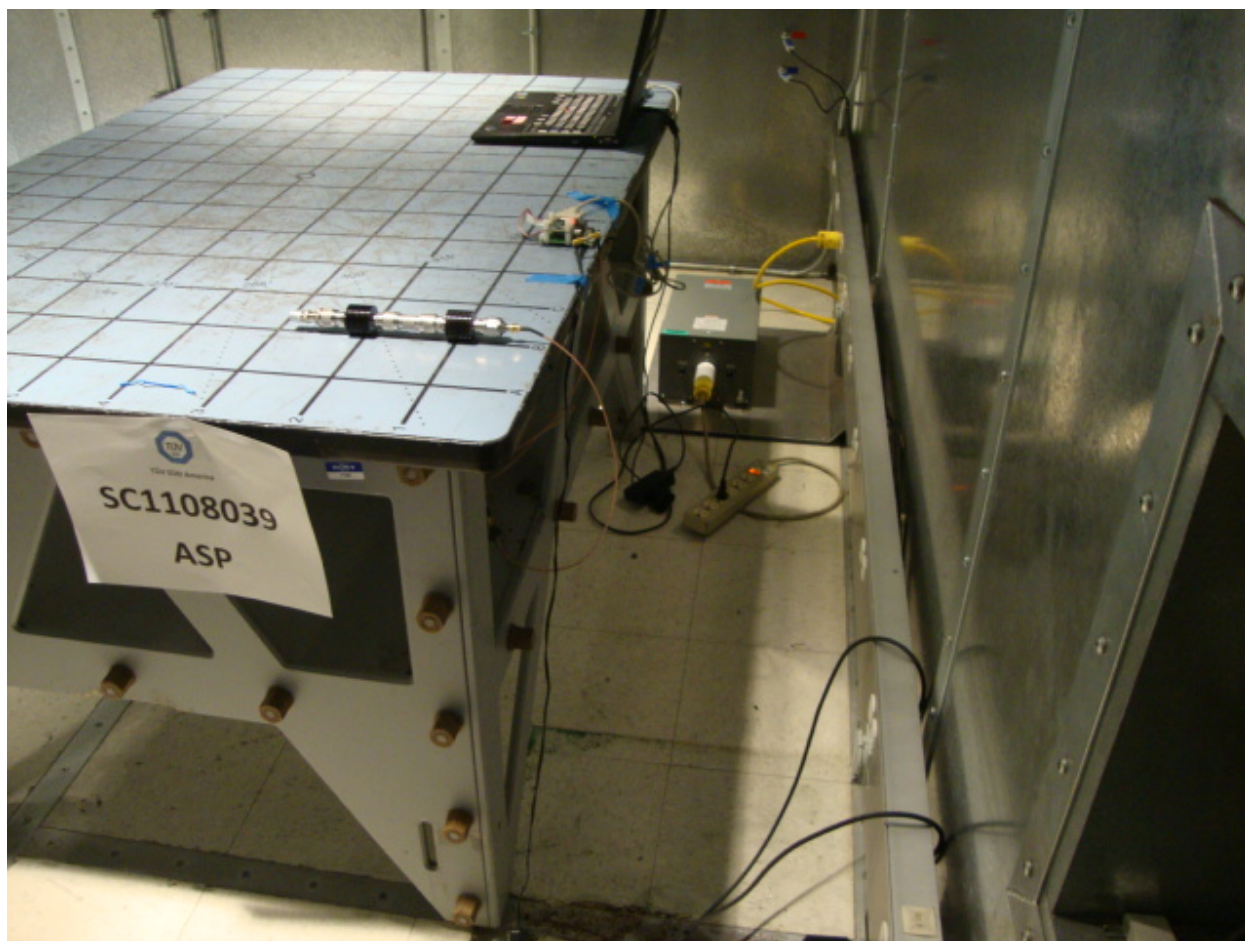
Conducted Emission Test Setup (Back)
