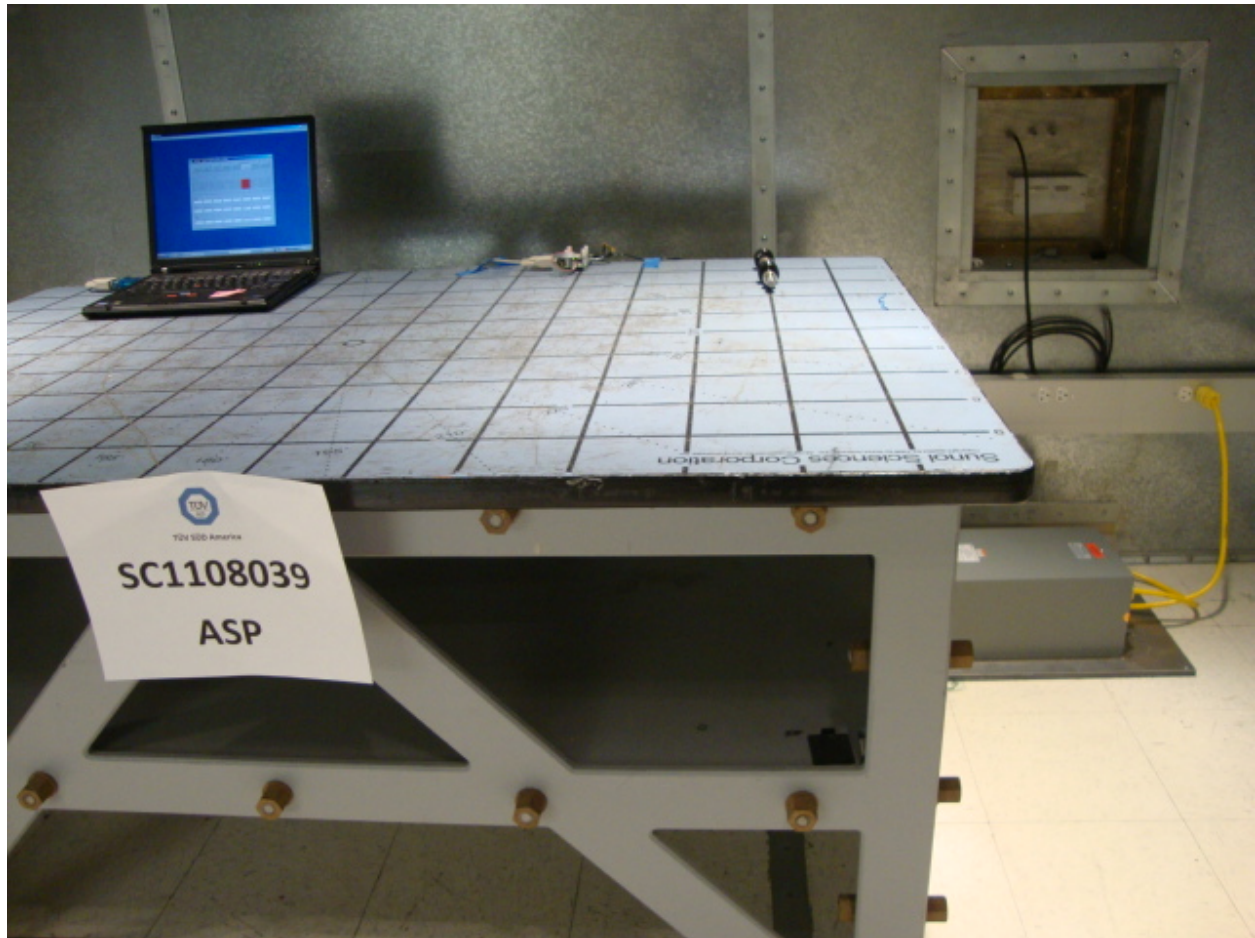
Conducted Emission Test Setup (Front)
