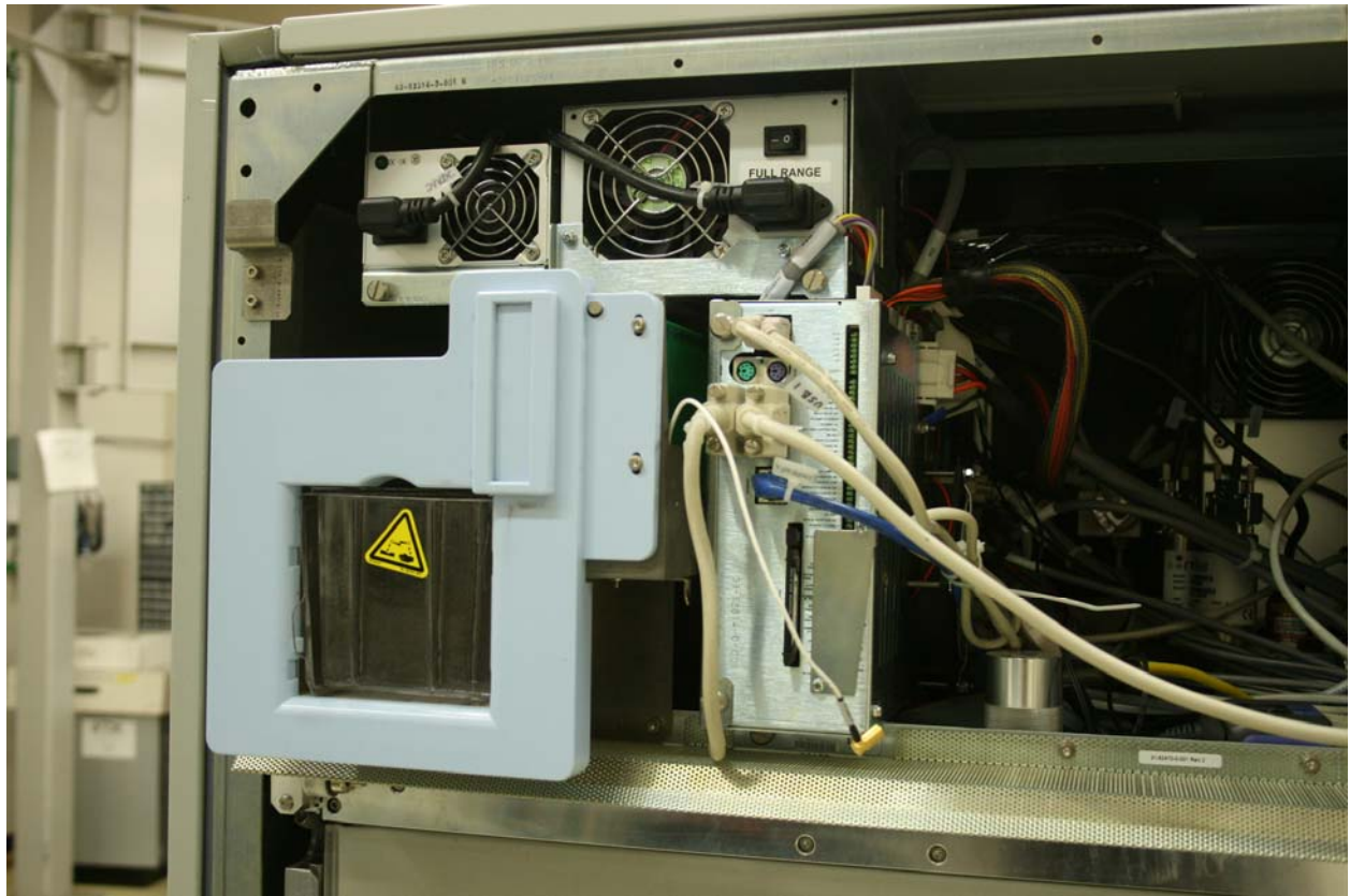
Front panel of EUT where STERRAD® 100NX™ Cassette is loaded and verified by the RFID system
