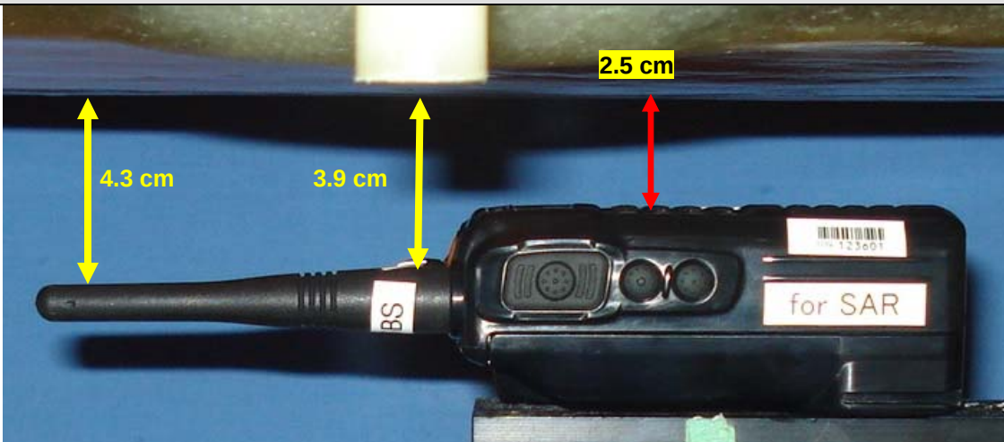
Face-held SAR Configuration - Antenna 2, Battery b
