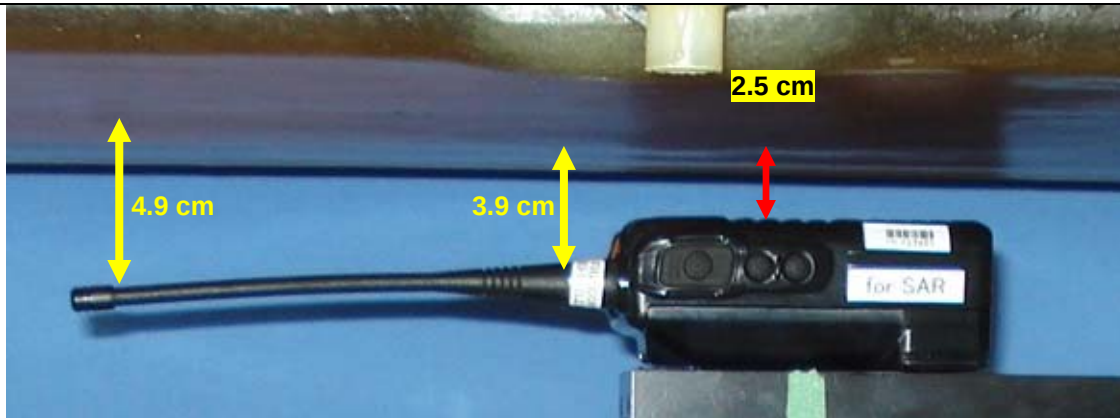
Face-held SAR Configuration - Antenna 1, Battery b
