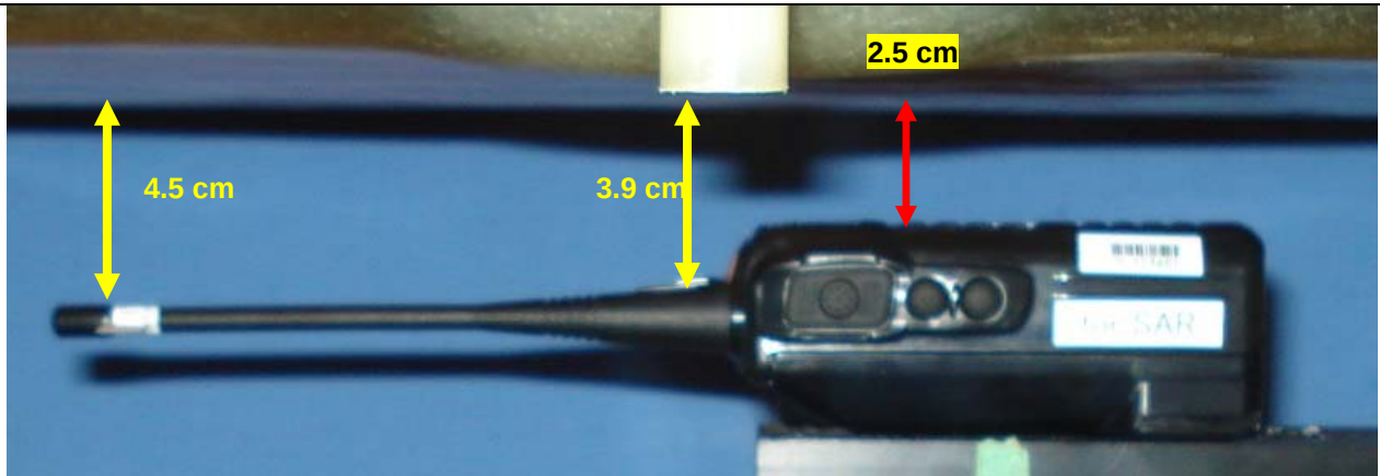
Face-held SAR Configuration - Antenna 4, Battery b
