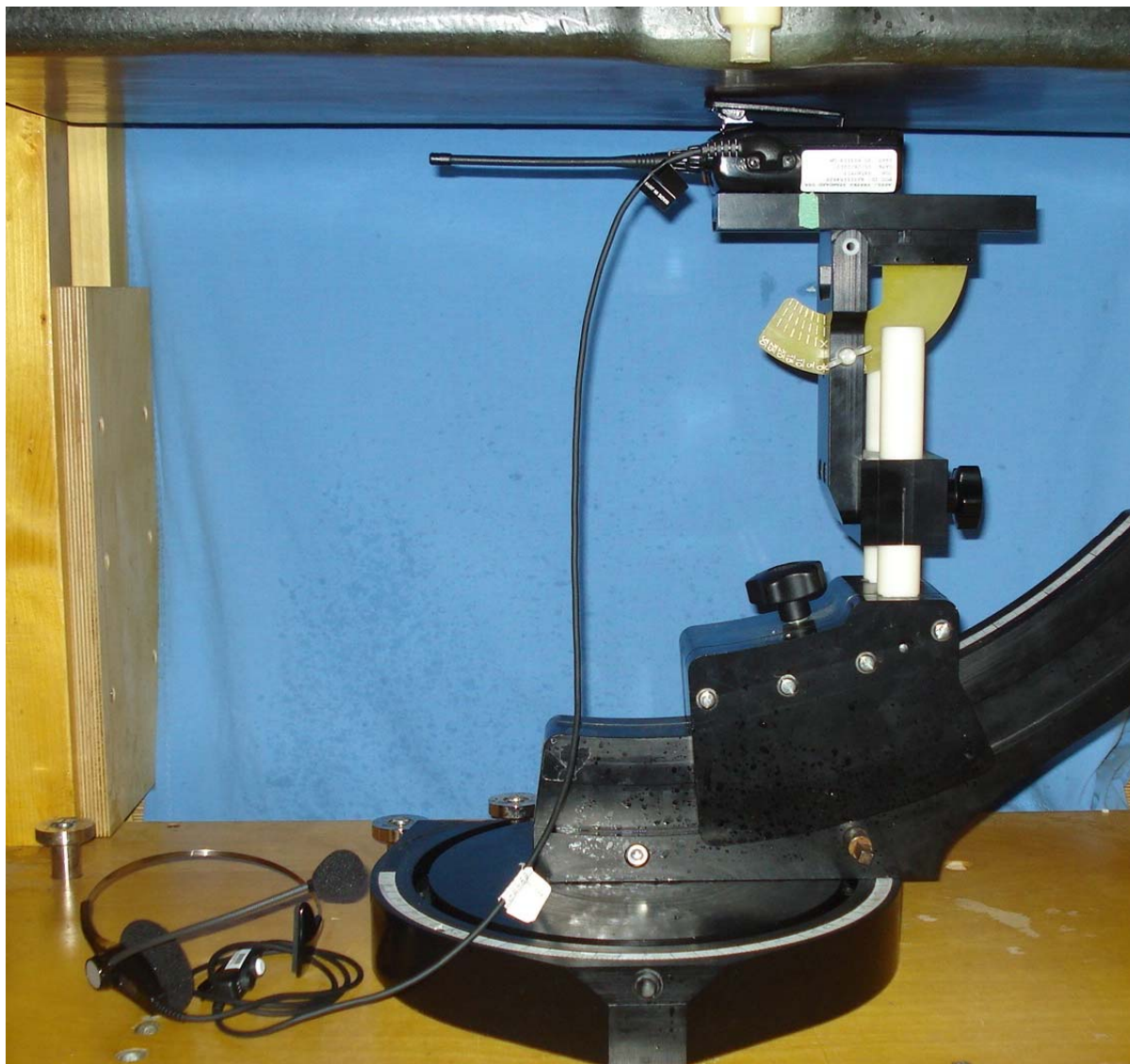
Body-worn SAR Configuration Test Setup
