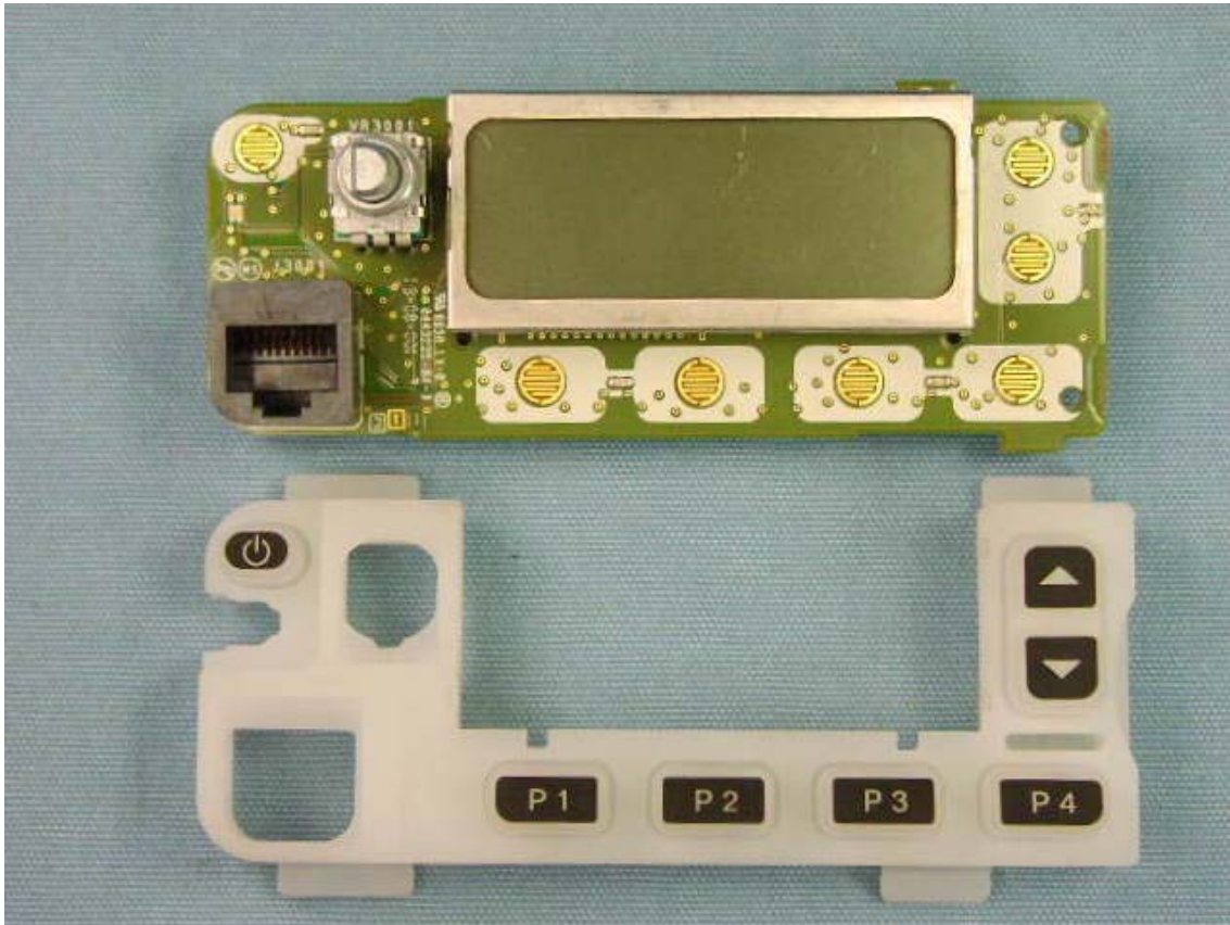
Side-A of FRONT-Unit and Rubber Key top (EVX-5400)
