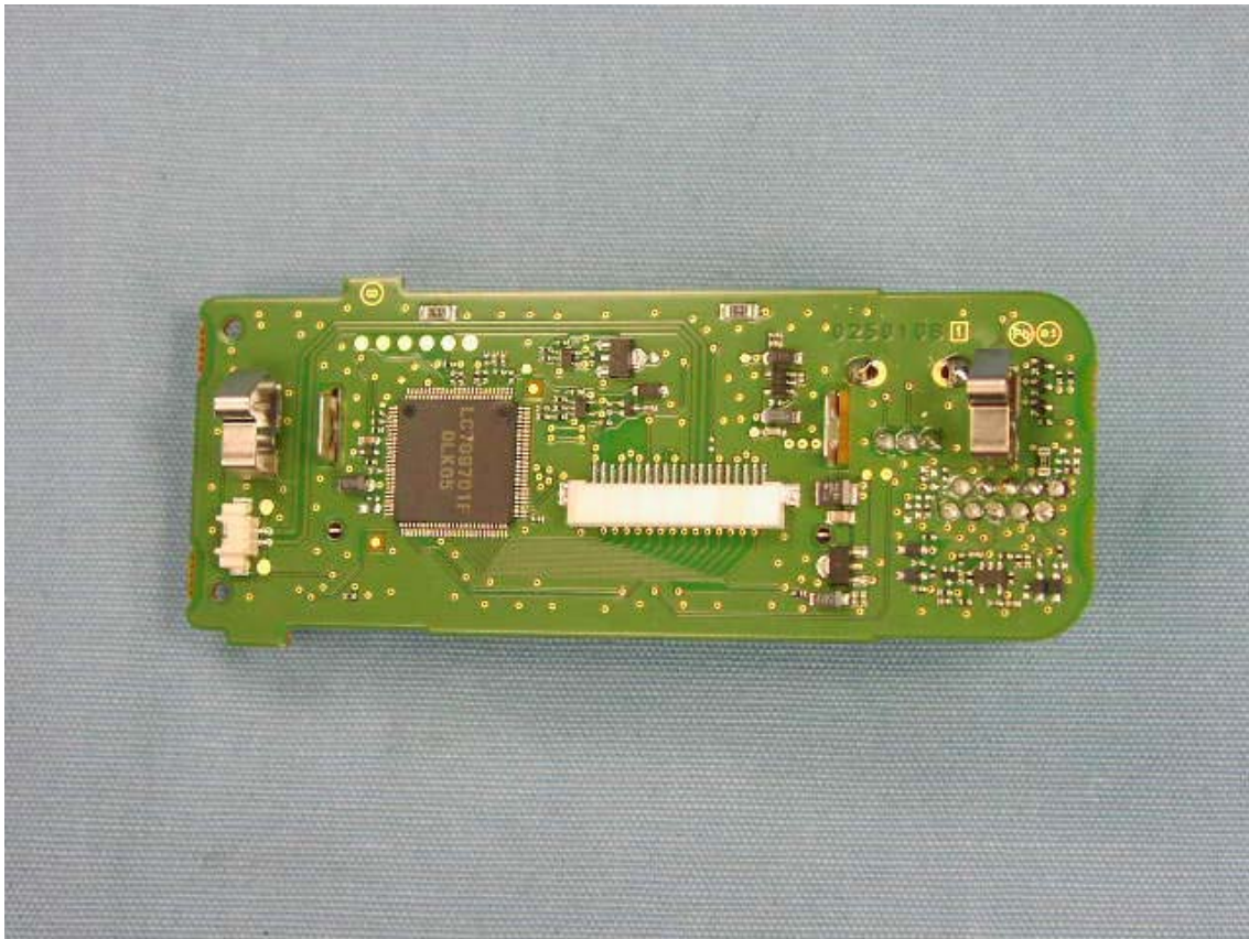
Side-B of FRONT-Unit (EVX-5400)
