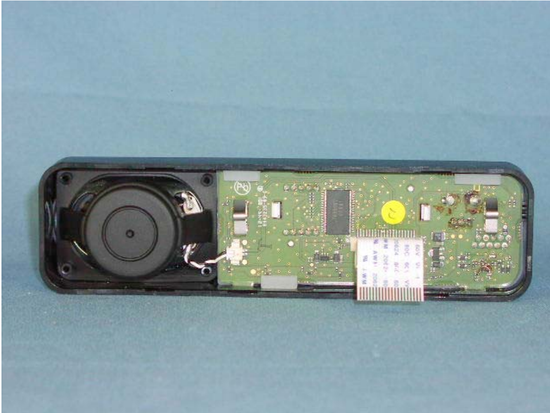
Inside of FRONT panel with Unit and SP (EVX-5300)
