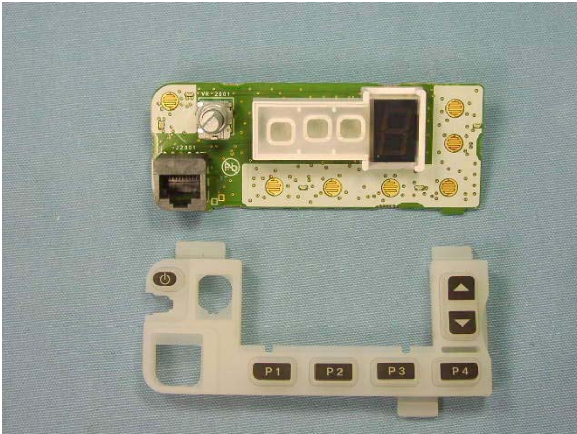
Side-A of FRONT-Unit and Rubber Key top (EVX-5300)
