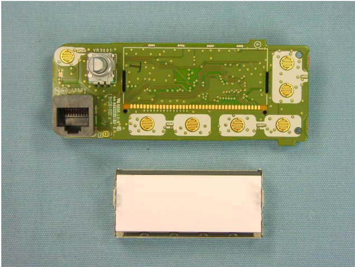
Side-A of FRONT-Unit Without LCD (EVX-5400)
