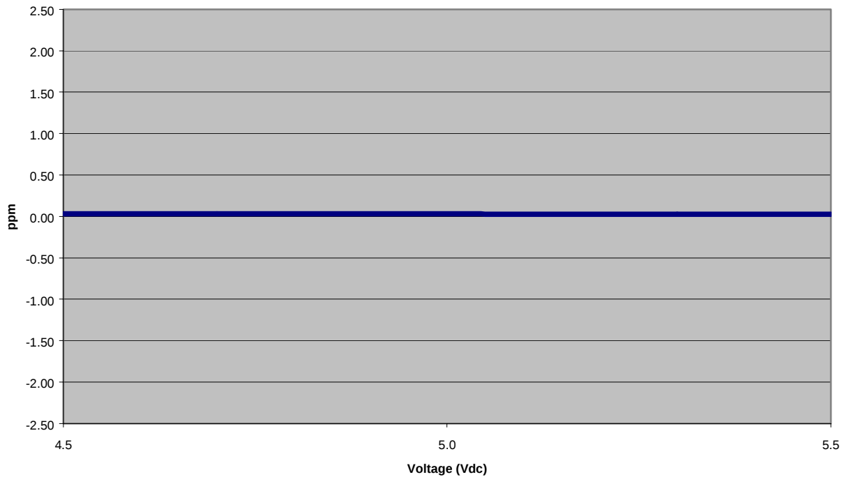
AMPS 800 Frequency Stability vs. Voltage (5 VDC Nominal) Carrier Frequency = 836.52 MHz Maximum Power Level (1.5 Watt)
