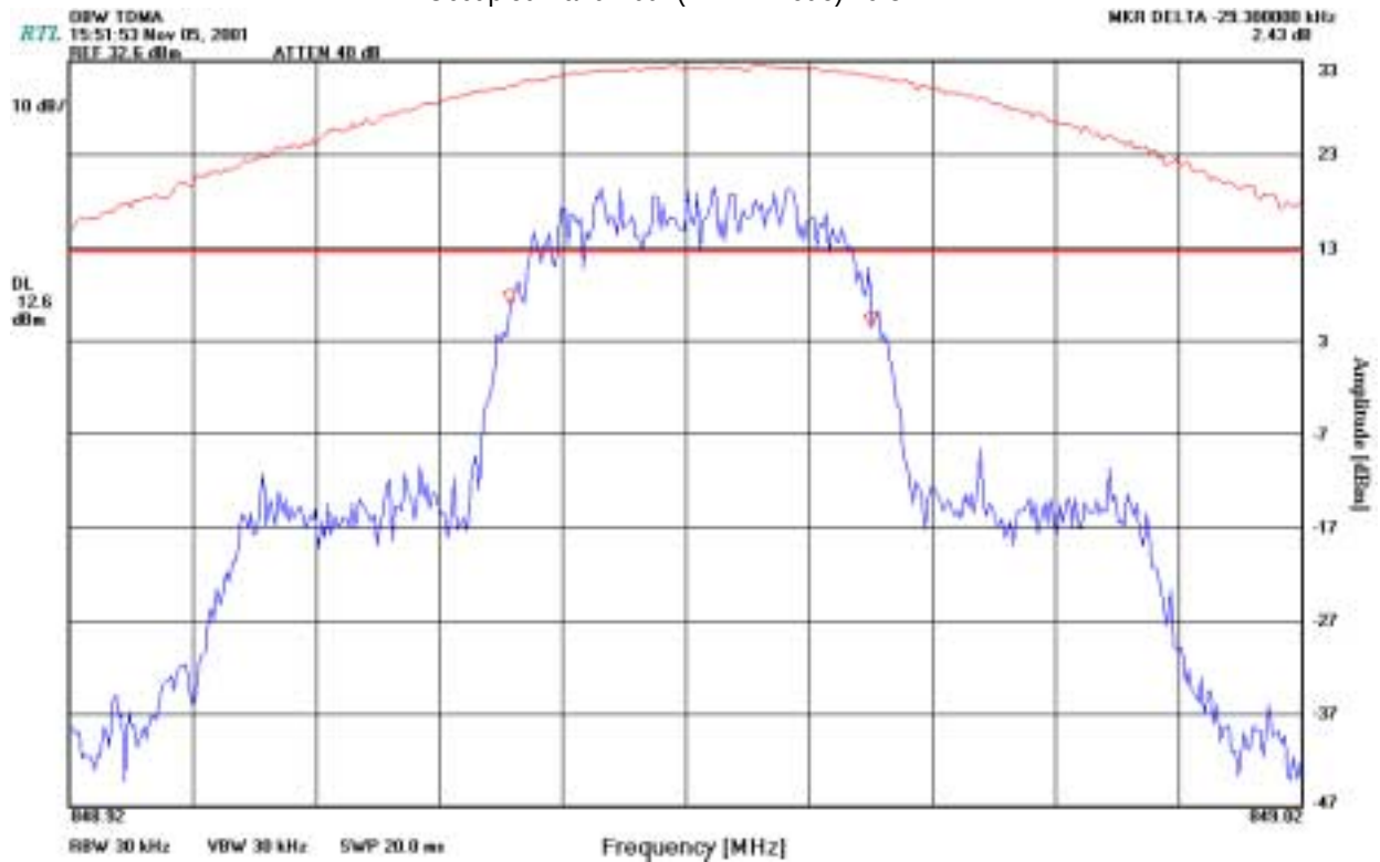
Occupied Bandwidth (TDMA mode) 29.3 KHz
