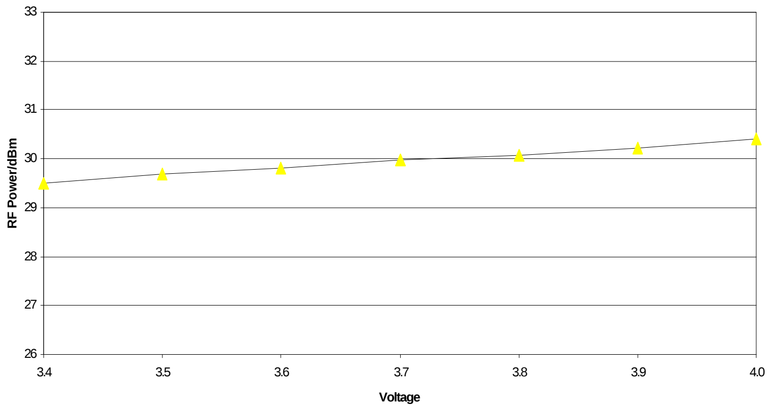
RF power across PCS band @ PL0 vs. Voltage
