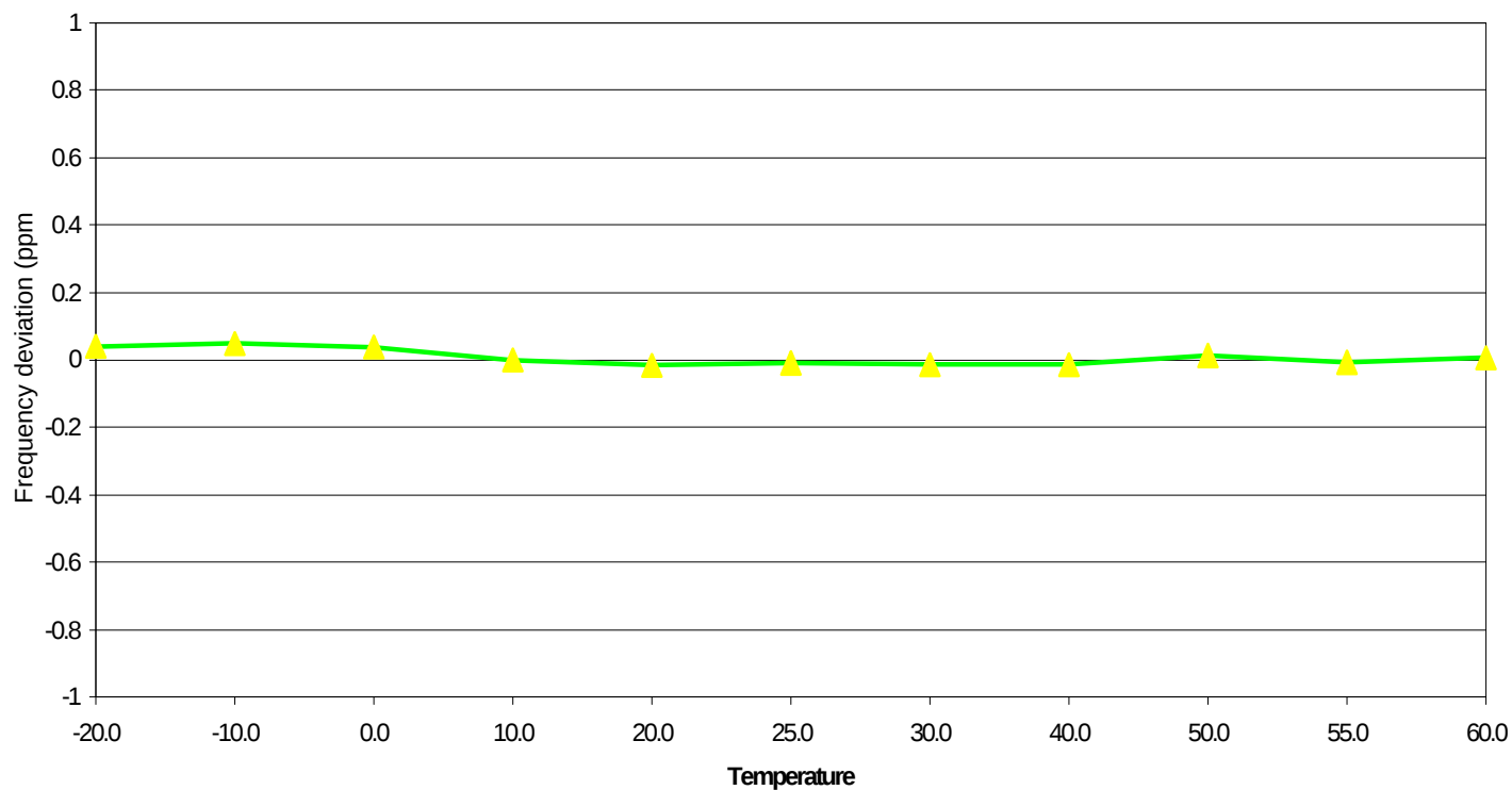
Frequency vs. Temperature
