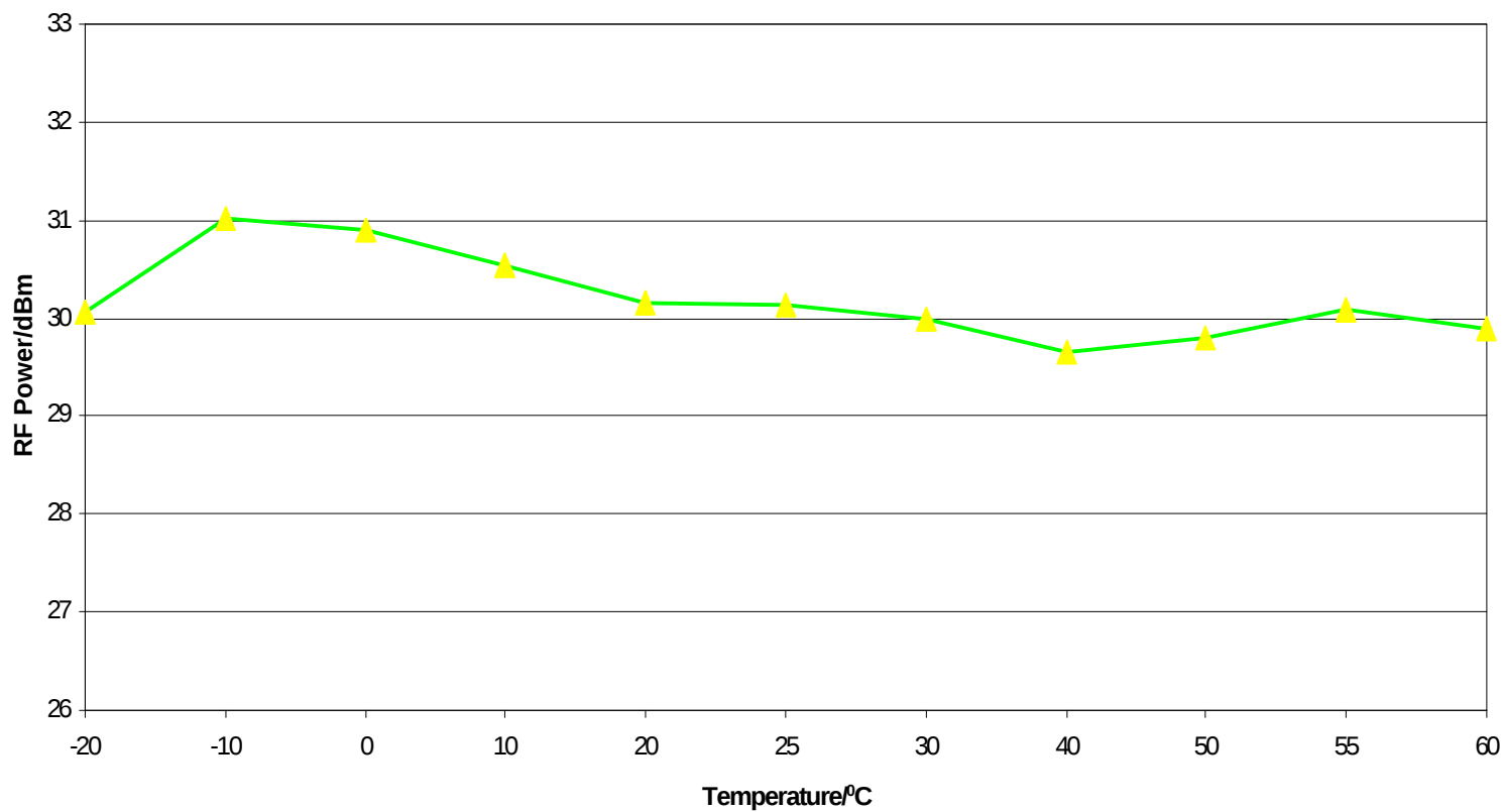
RF power across PCS band @ PL0 vs. Temperature
