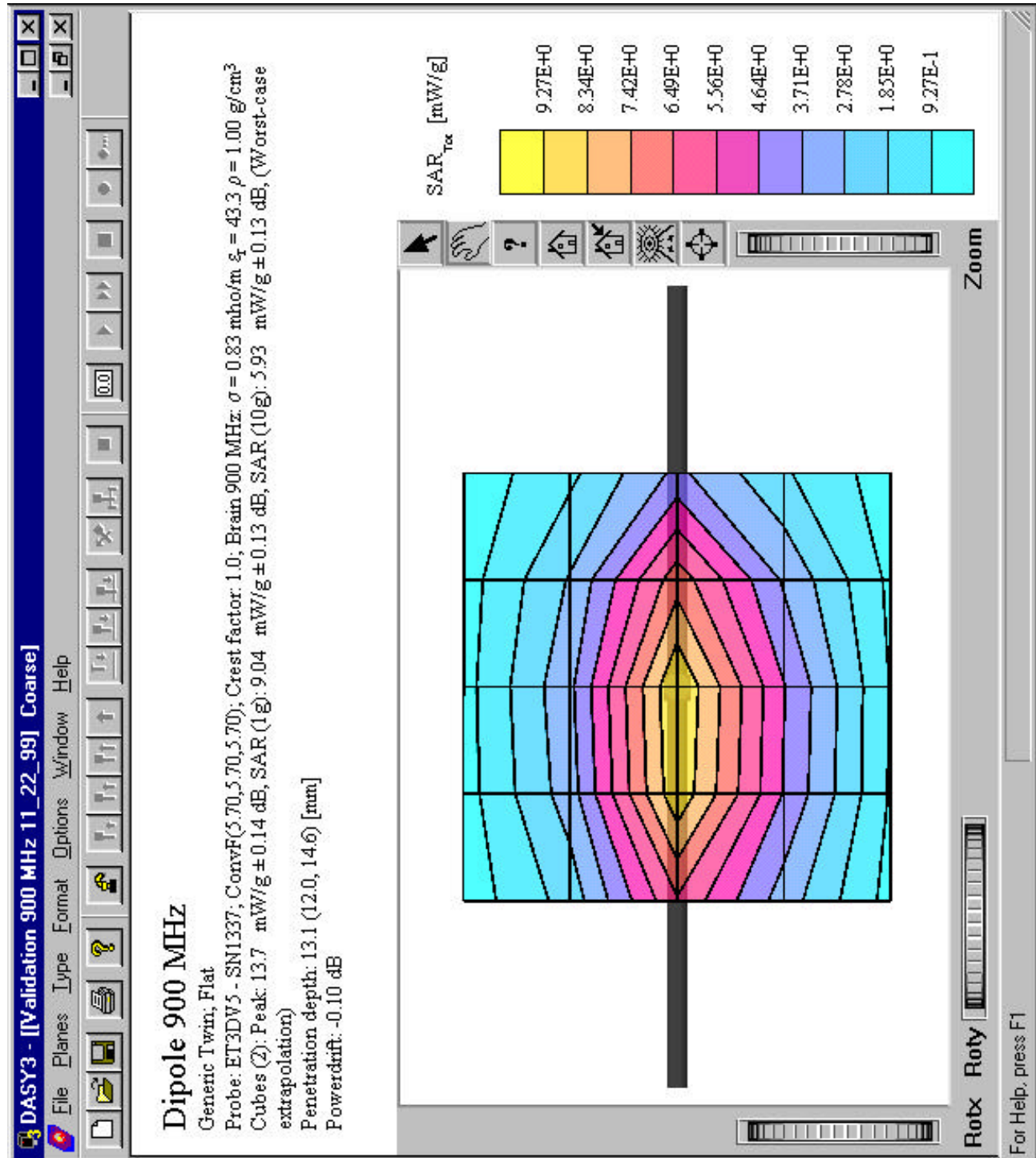
900 MHz SAR distribution of validation dipole antenna from system accuracy verification test.
