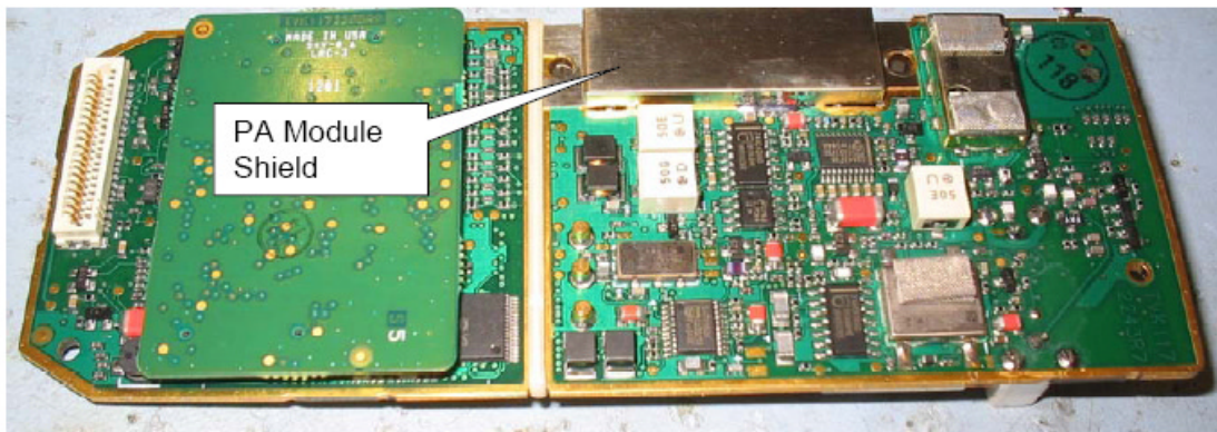
Front of Main Board
