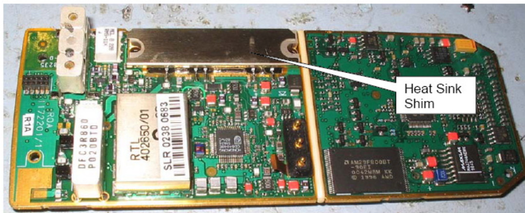
Back of Main Board
