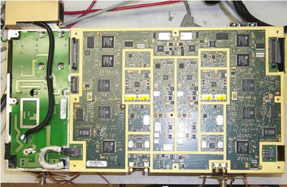
Example 3 Top View of Power Supply and TRX Boards
