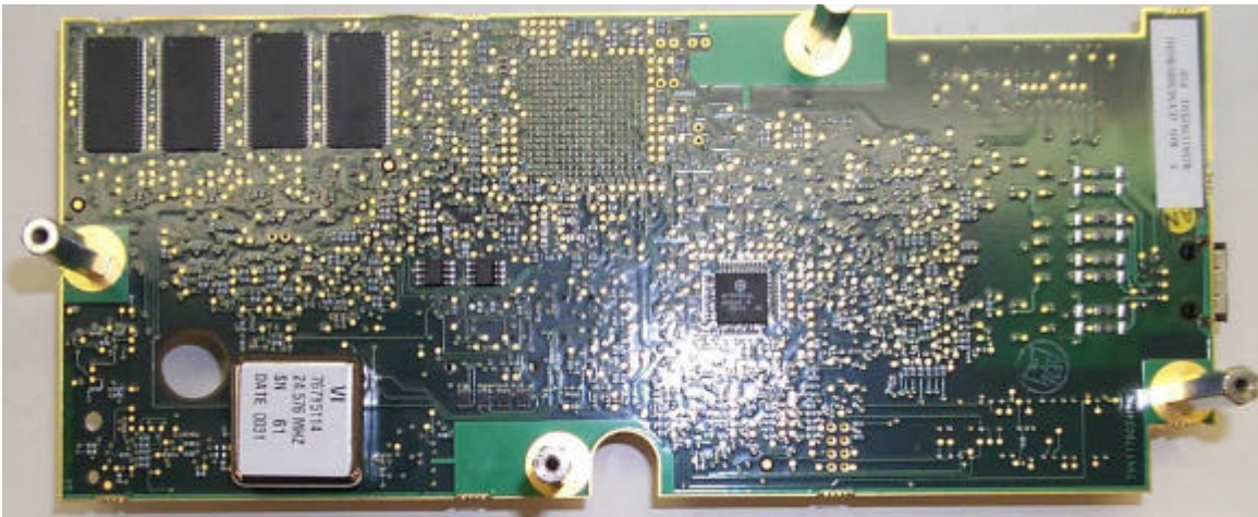
Example 2 Bottom View of RHI Board
