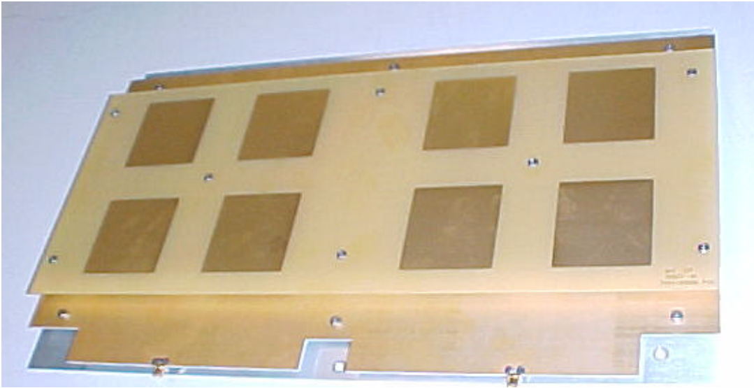
Top side of Patch antenna
