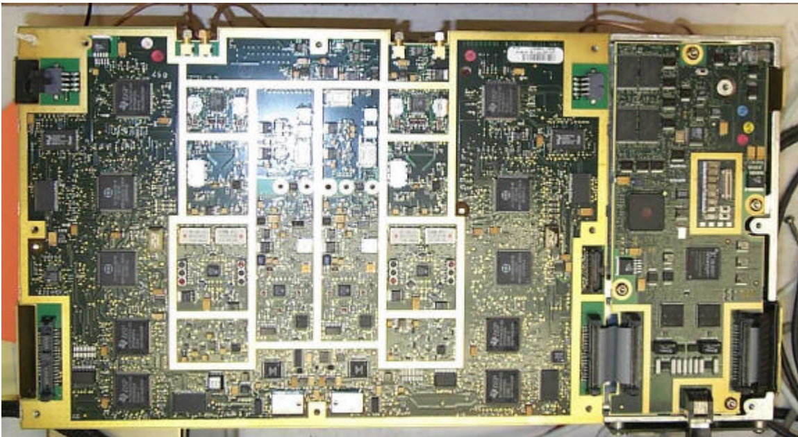
Example 4 Top View of RHI and TRX Boards
