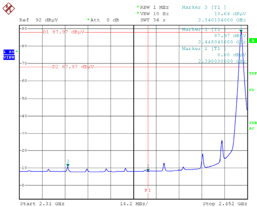
Band edges-fL
