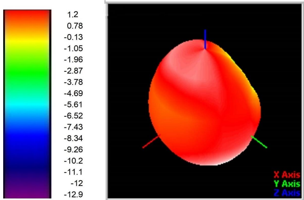
3D radiation pattern diagram frequency range: 2440MHz Unit:dBi
