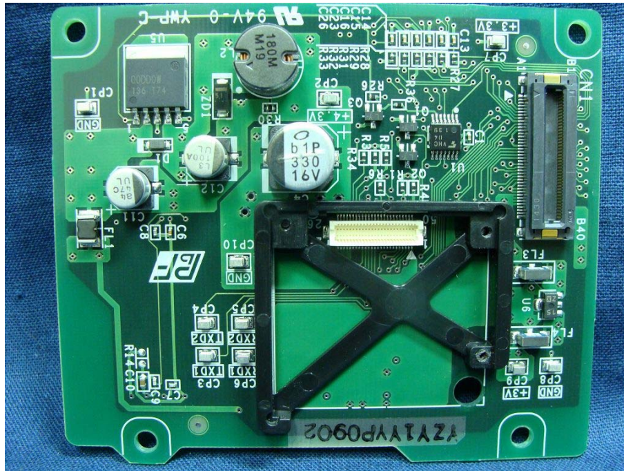
(11) EUT Photo
