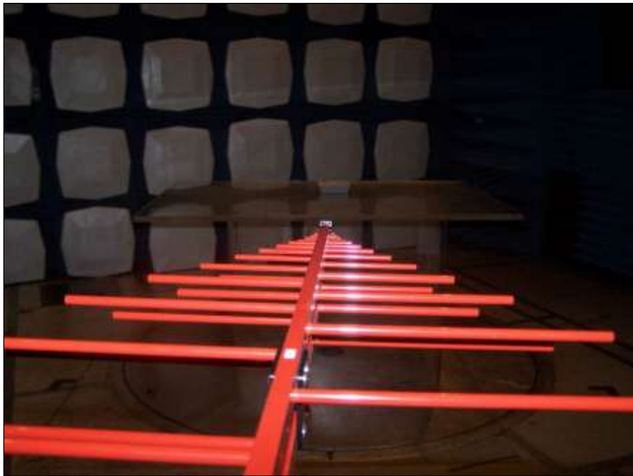
Photograph 3. Radiated Emissions, Test Results, Batteries Only
