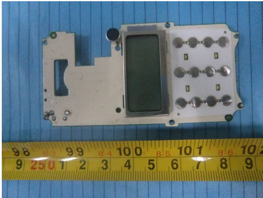
EUT – Key Board Top View (Model: PX-568V)
