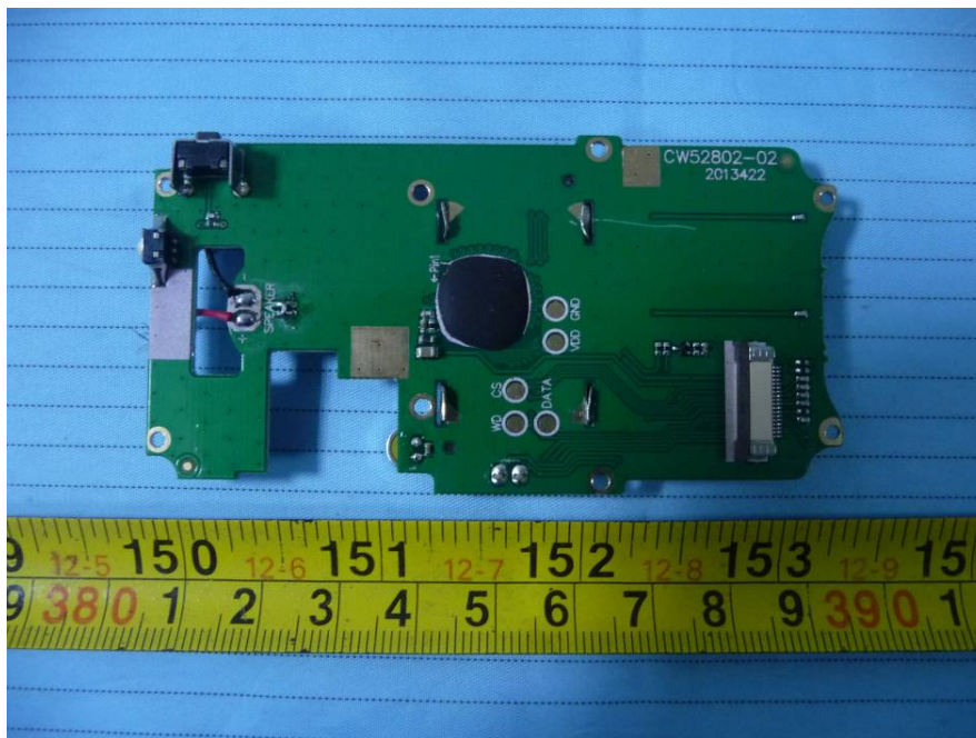
EUT – LCD Board Bottom View (Model: PX-578V)
