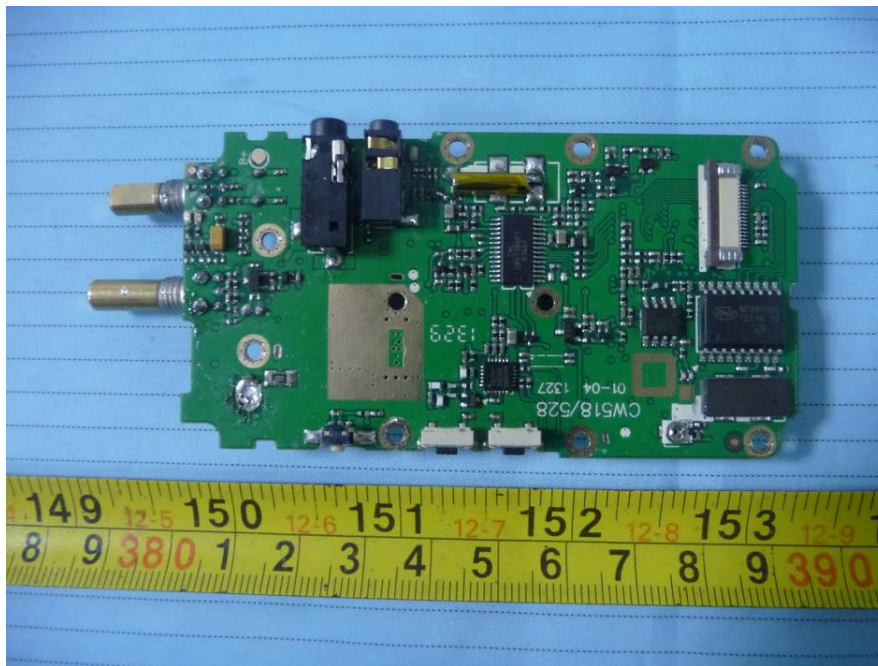
EUT – Main Board Bottom View (Model: PX-578V)
