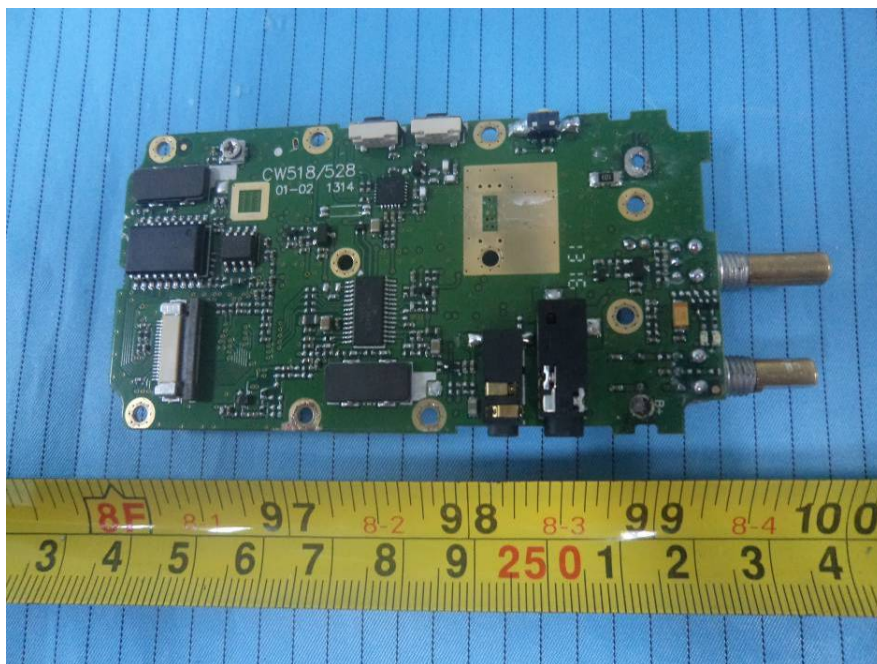
EUT – Main Board Bottom View (Model: PX-568V)
