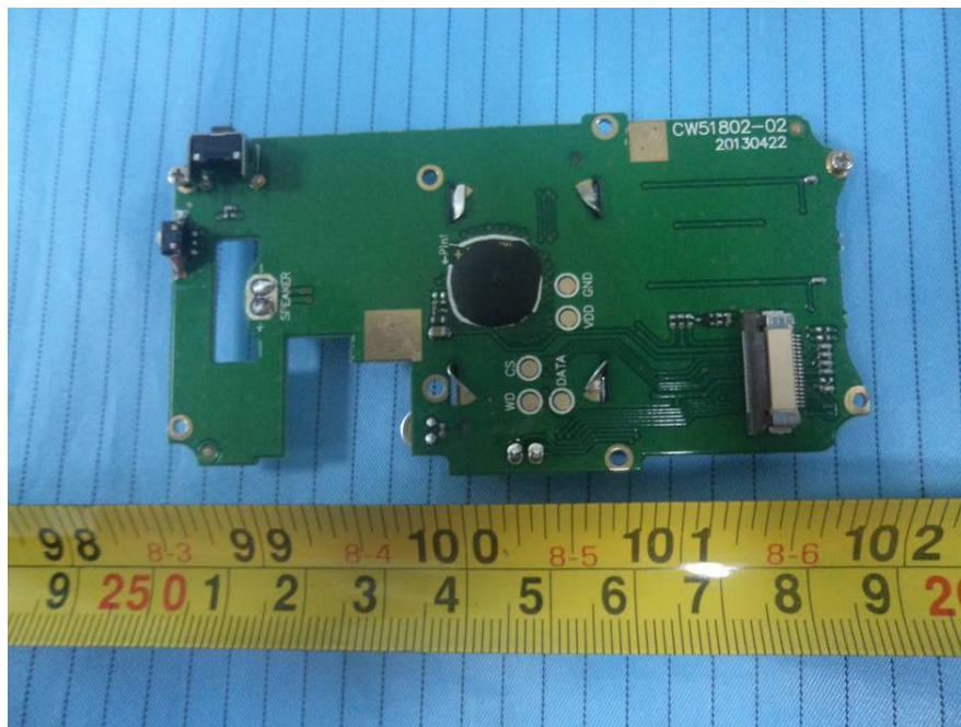
EUT – Key Board Bottom View (Model: PX-568V)
