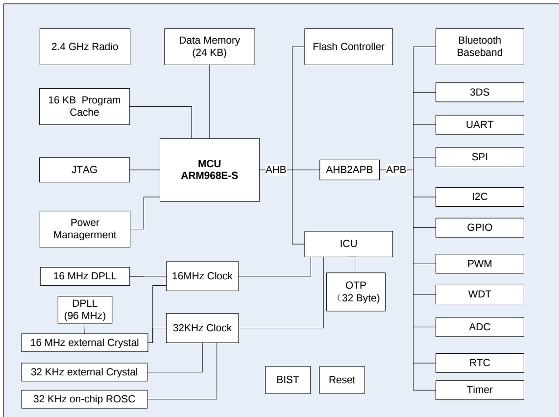
Figure 1 Block Diagram
