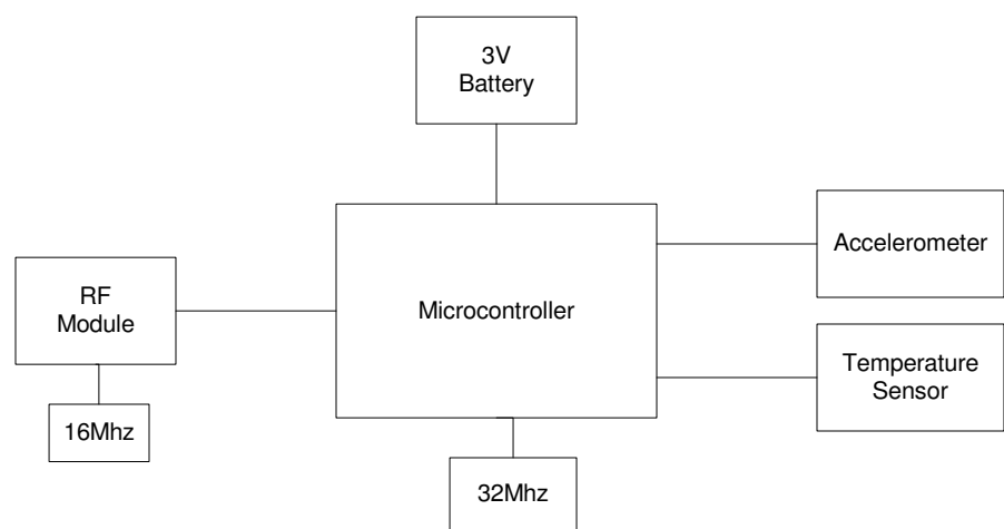
WSN Sensor Block Diagram, Rev1, Gorko Systems Inc.
