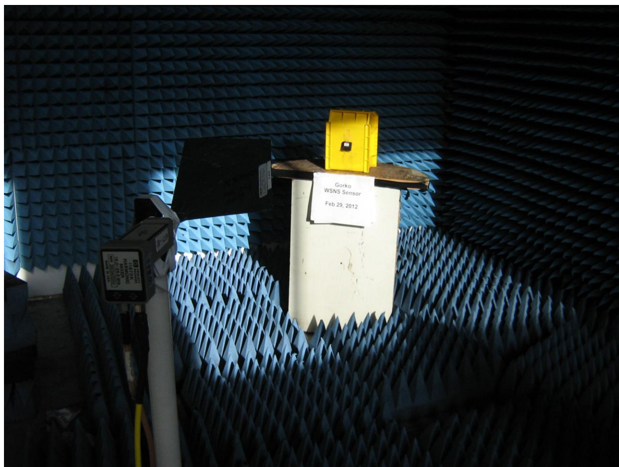
Test Setup for Spurious Radiated Emissions Frequencies above 18 GHz.
