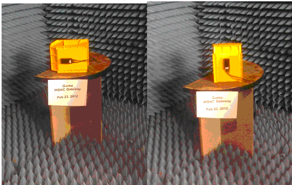
Test Setup for High Frequency Radiated Emissions (Horizontal and Vertical)
