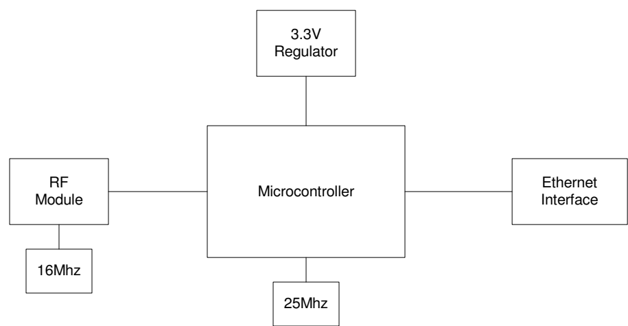
WSN Collector Block Diagram, Rev1 , Gorko Systems Inc.
