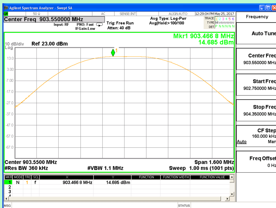
Antenna 2- Channel 1 (903.55MHz)
