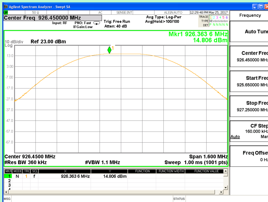
Antenna 2-Channel 55 (926.45MHz)
