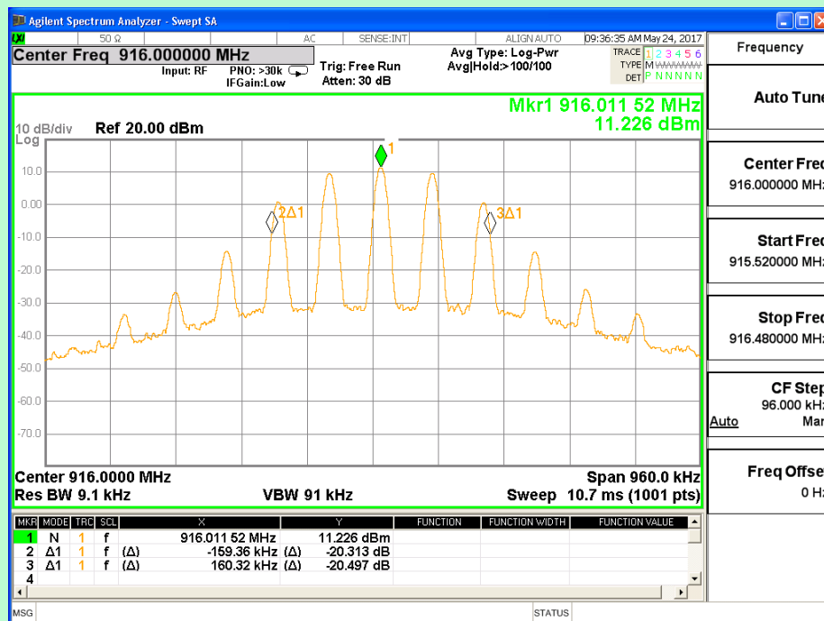
Channel 28 (916MHz)
