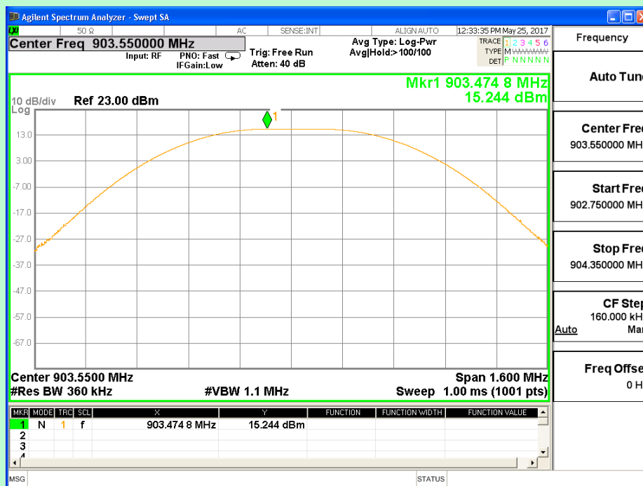
Antenna 3- Channel 1 (903.55MHz)
