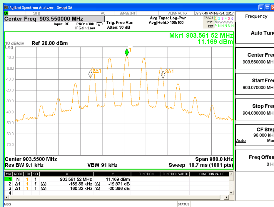
Channel 1 (903.55MHz)
