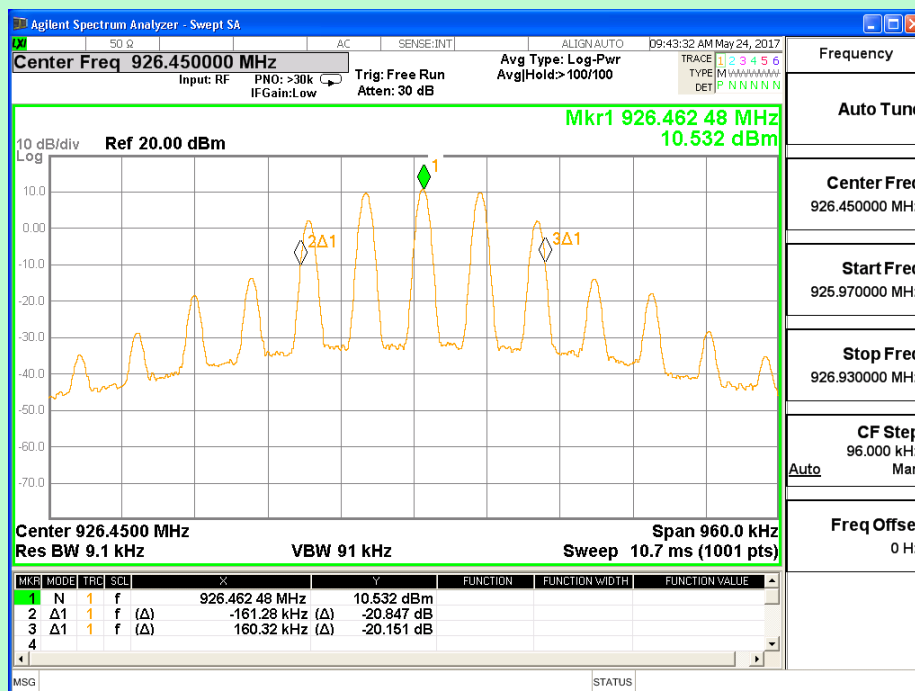
Channel 55 (926.45MHz)
