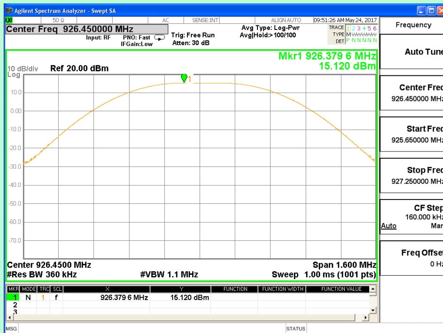
Antenna 1-Channel 55 (926.45MHz)
