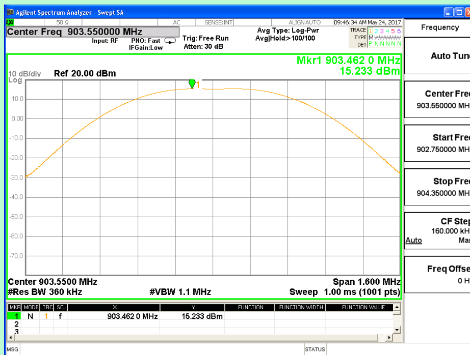
Antenna 1- Channel 1 (903.55MHz)
