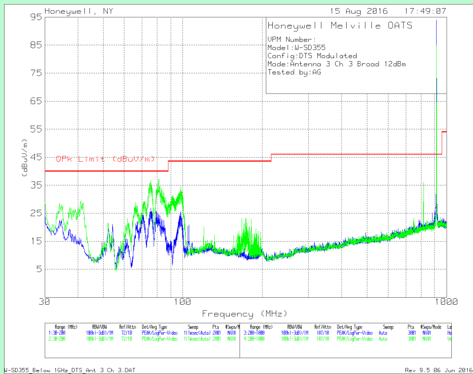
Channel 3 (914.325 MHz) – Antenna 3
