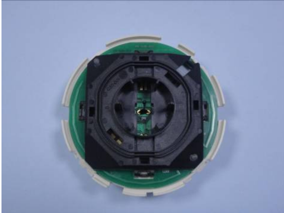
Heat Smoke Detector – Internal Photo – 1
