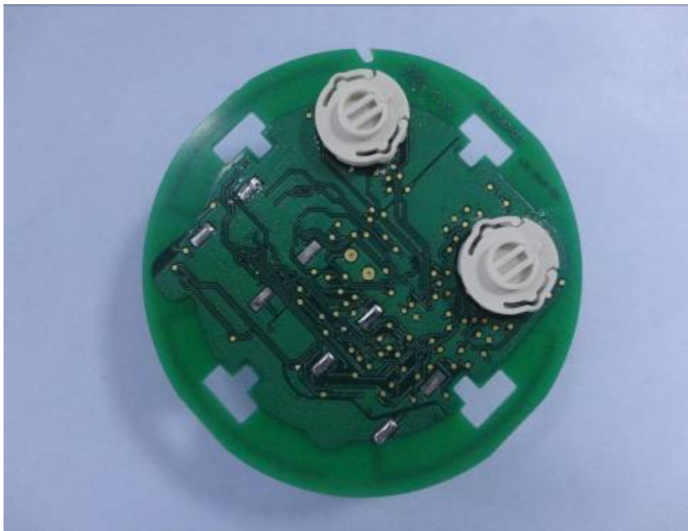
Acclimate / Photo Heat Smoke Detector - PCB –Bottom View
