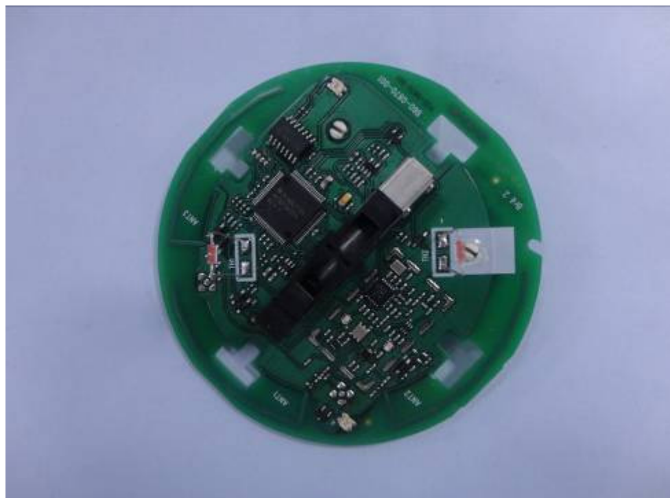
Acclimate / Photo Heat Smoke Detector - PCB – Top View
