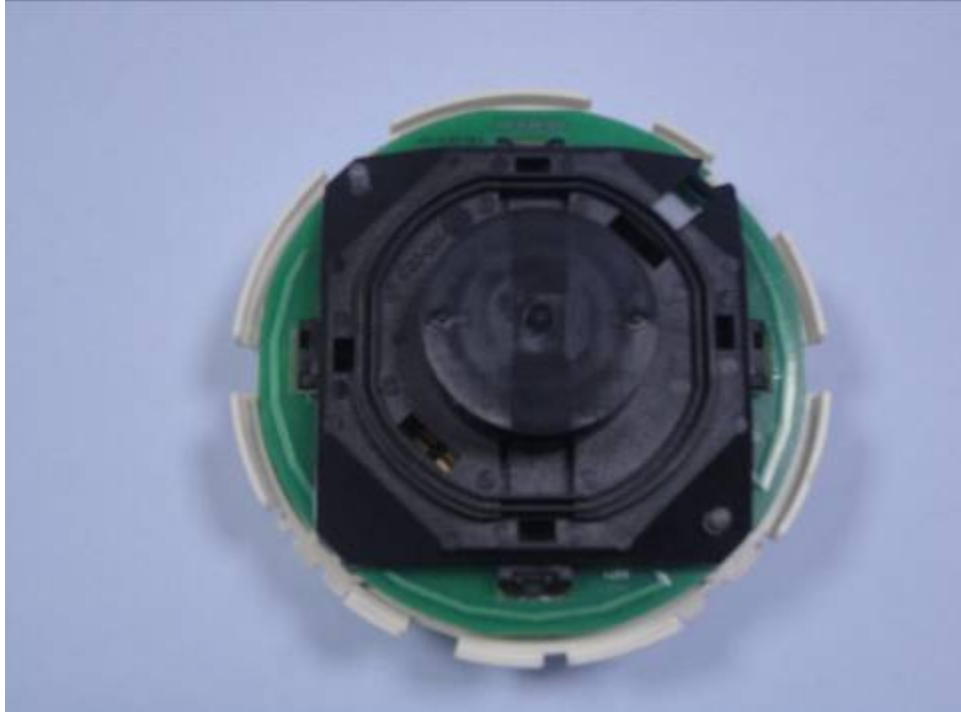
Photo Smoke Detector – Internal Photo – 1
