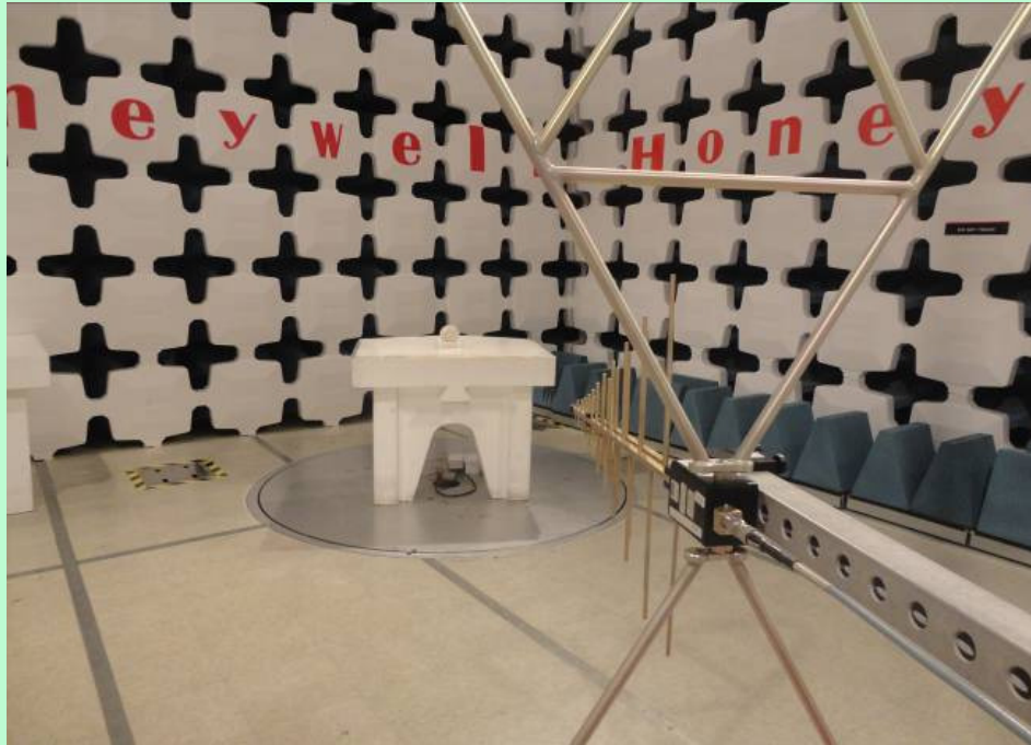
Radiated Emission Setup –30 MHz to 1 GHz [ Horizontal Polarization ]
