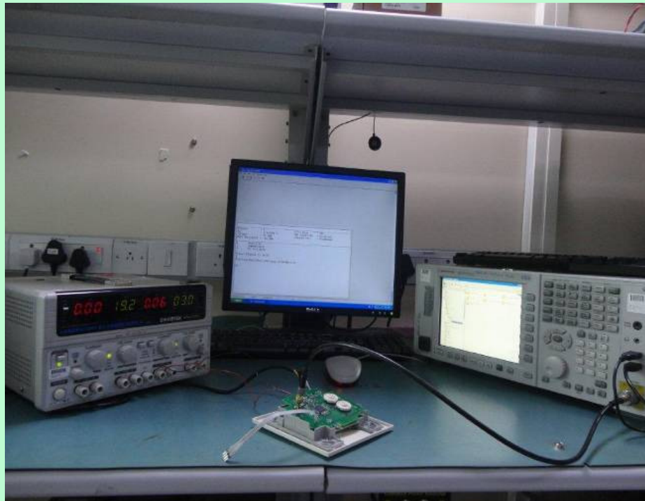
Conducted RF Test Setup
