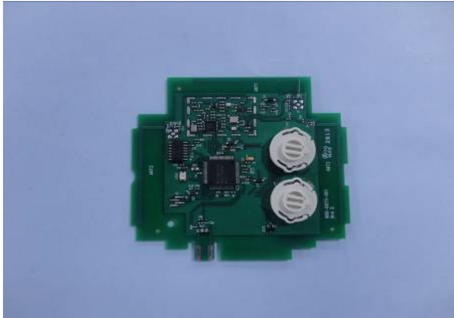
PCB – Top View
