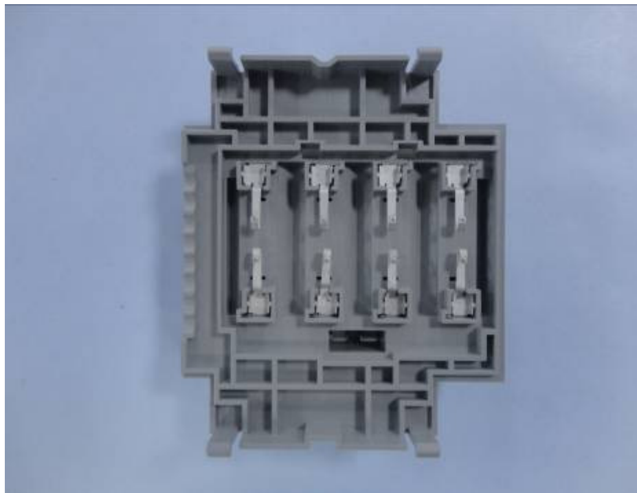
Internal Bottom Cover
