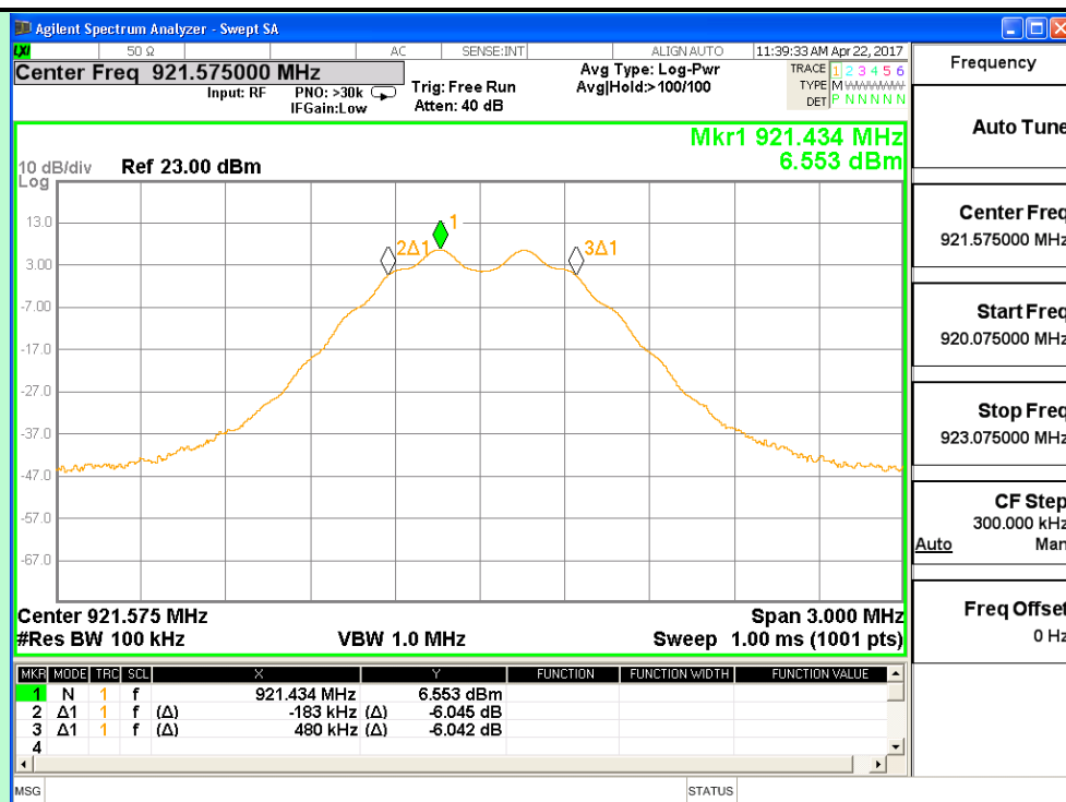
Channel 5 (921.575MHz)
