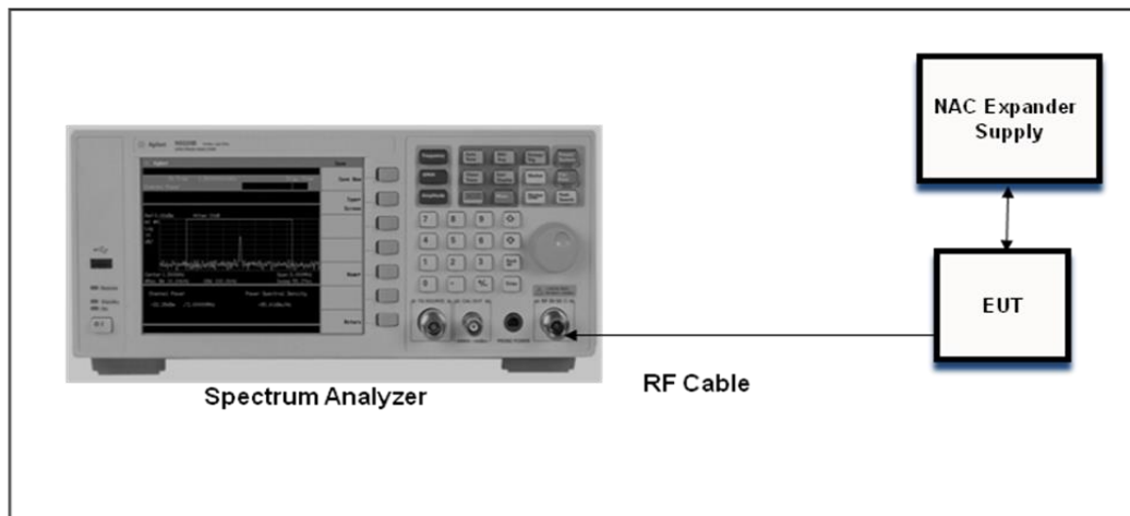
Conducted RF Test Setup
