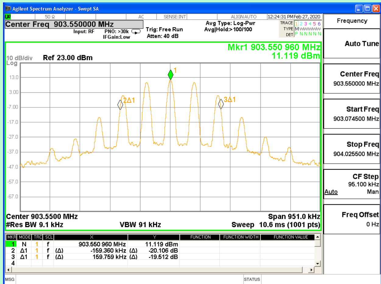
Channel 1 (903.55MHz)
