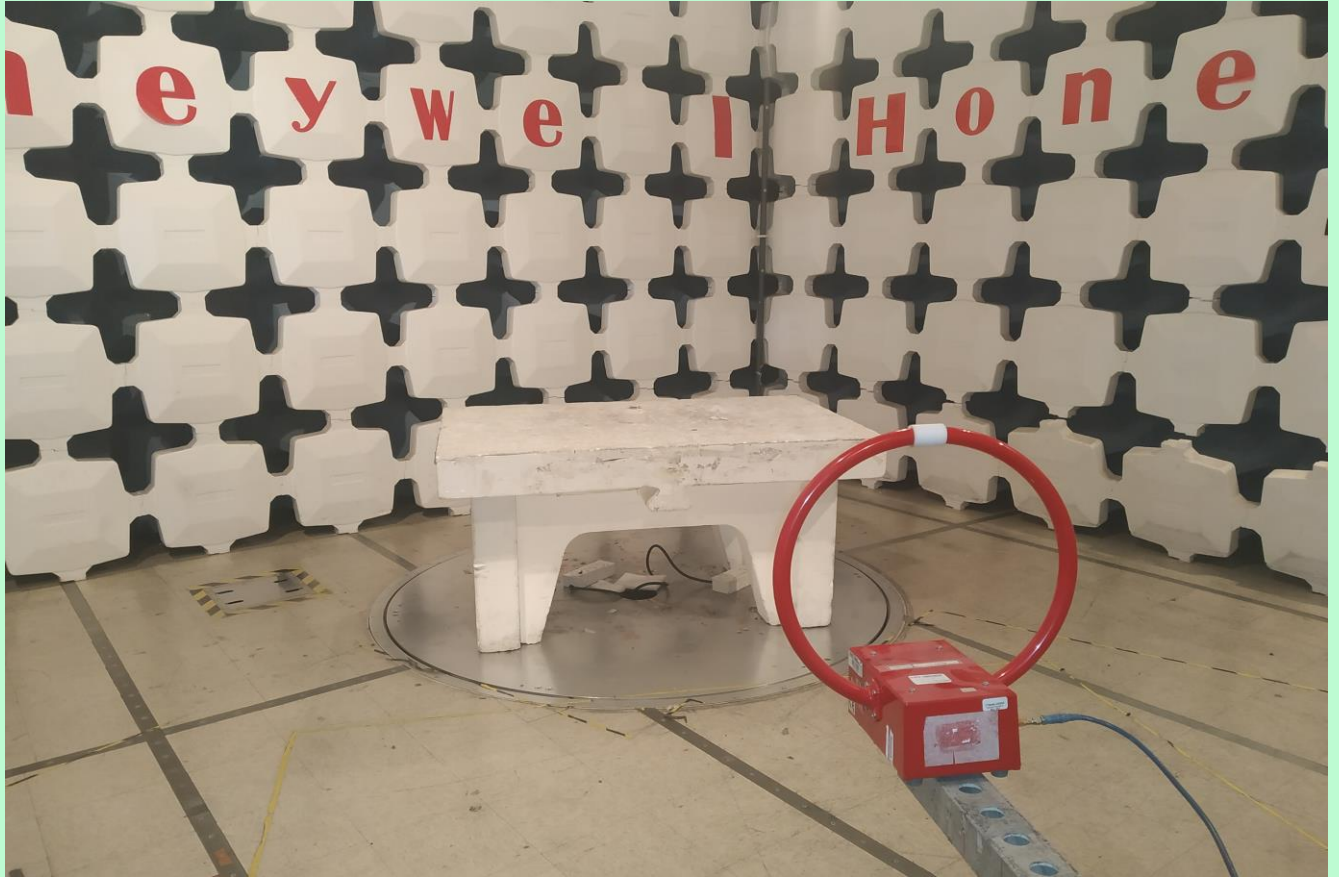
Radiated Emission Setup – 9 KHz to 30 MHz [ Parallel ]
