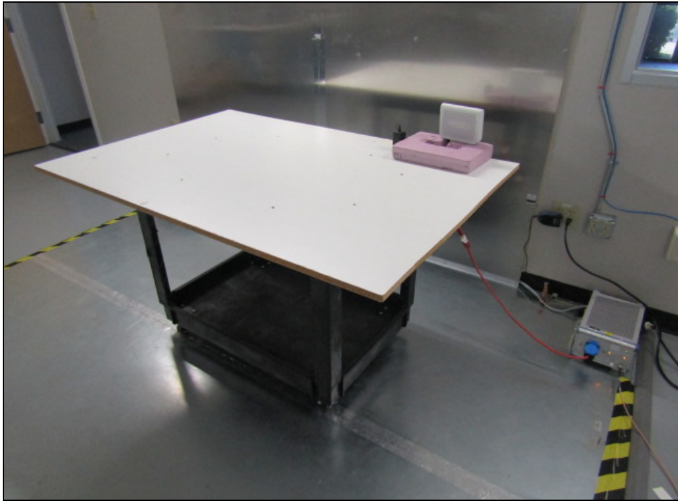
Figure 1: Powerline Conducted Emissions - Front
