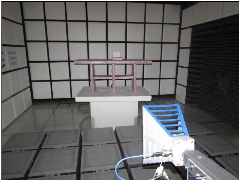
Figure 3: Radiated Emissions Above 1GHz - Front
